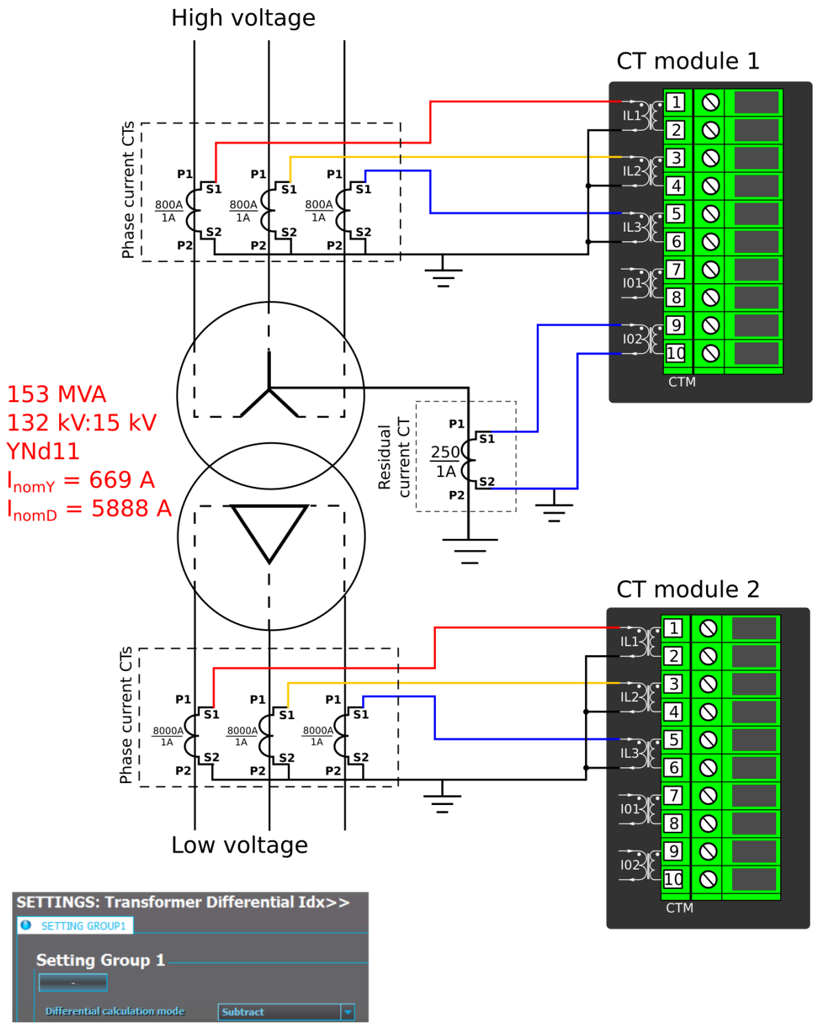
Figure. 5.2.1 - 4. Connections (application 1).
