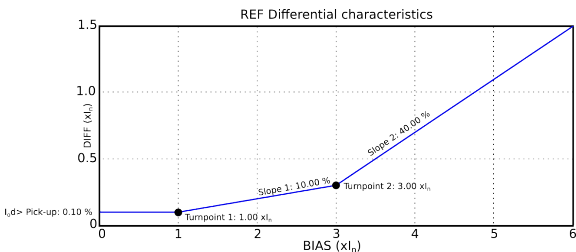
Figure. 5.4.9 - 57. Differential characteristics for the I 0d > function with default settings.
