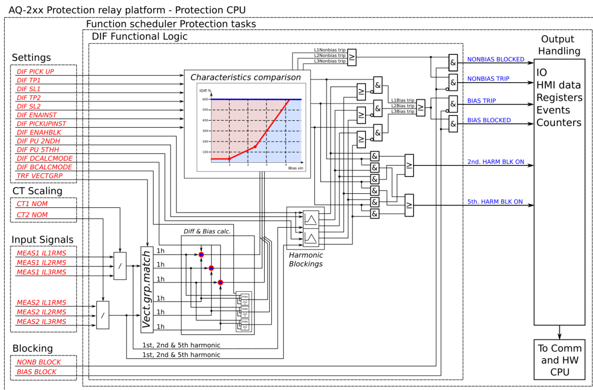
Figure. 5.4.21 - 129. Simplified function block diagram of the transformer differential function.
