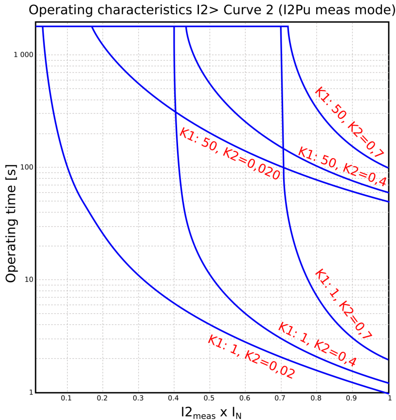
Figure. 5.4.6 - 43. Operation characteristics curve for I_2 > Curve2.
