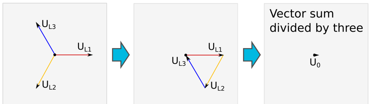
Figure. 5.4.12 - 74. Normal situation.
