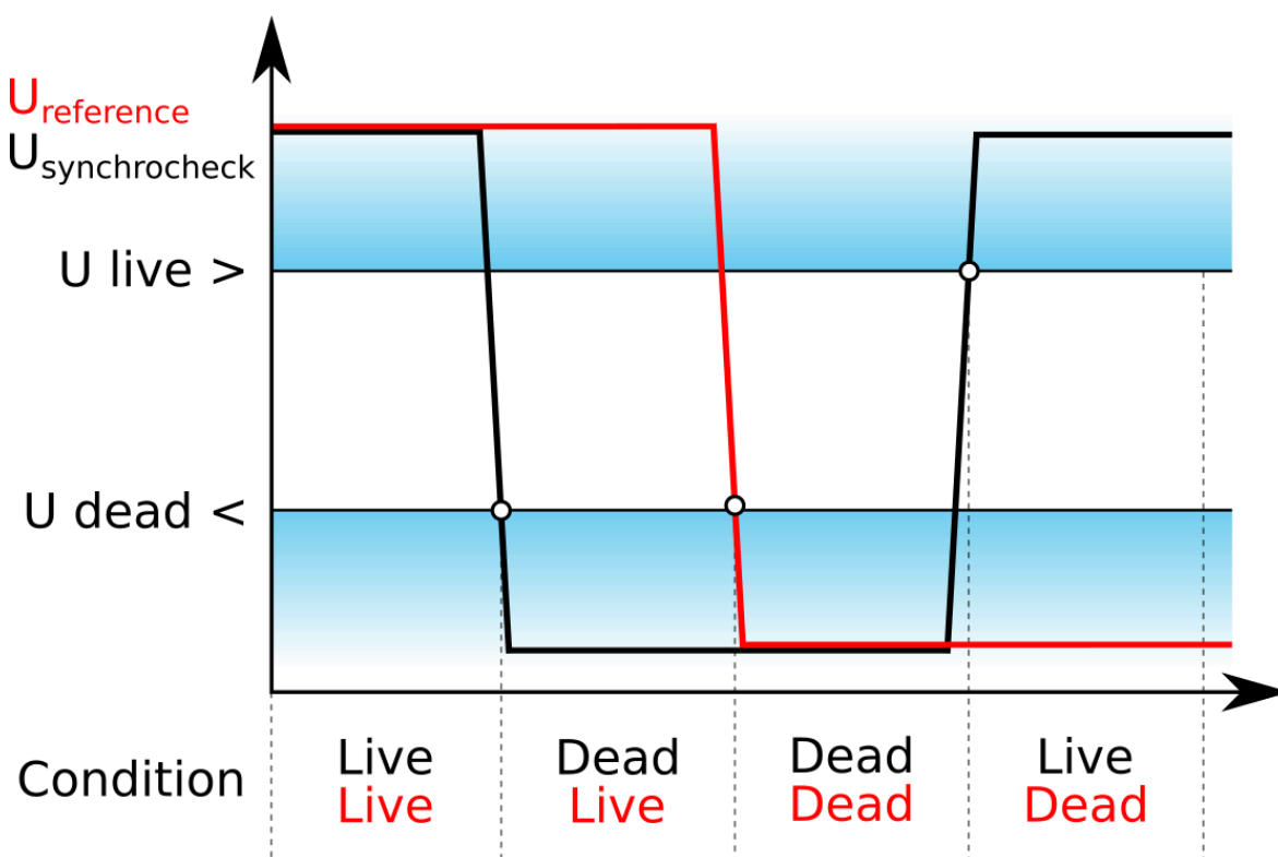
Figure. 5.5.6 - 169. System states.
