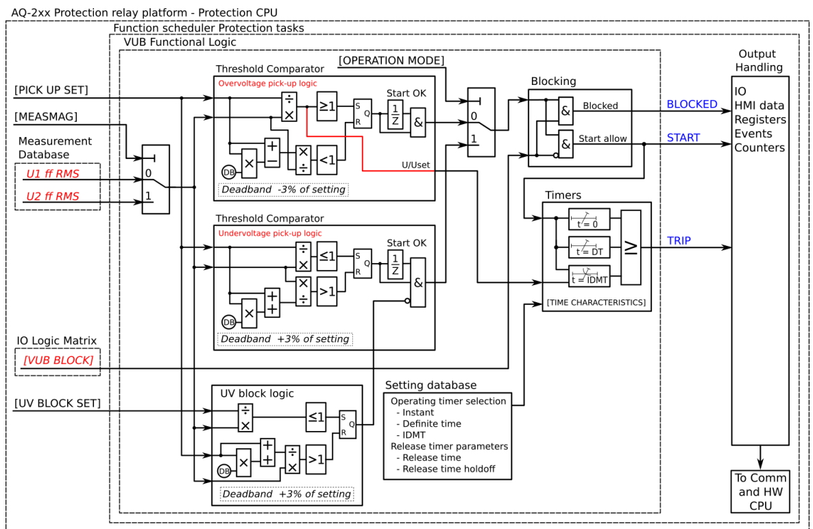
Figure. 5.4.13 - 84. Simplified function block diagram of the U1/U2>/< function.
