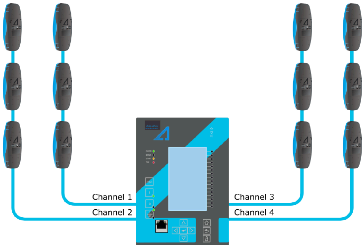
Figure. 5.4.23 - 131. IED equipped with arc protection.
