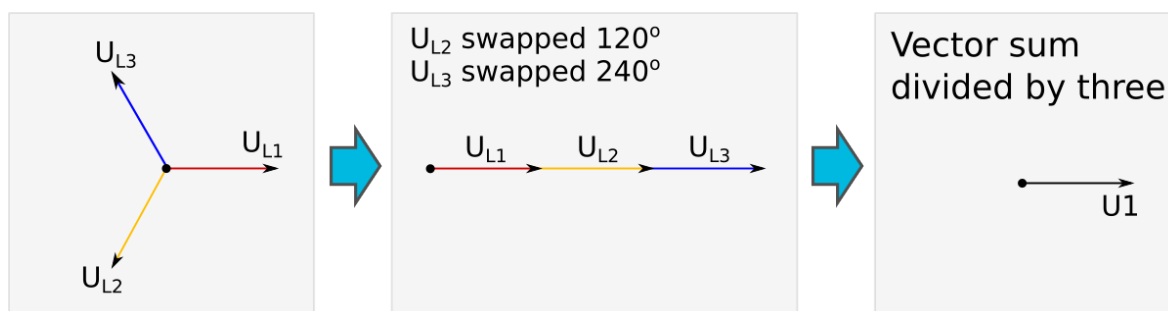
Figure. 5.4.13 - 78. Normal situation.
