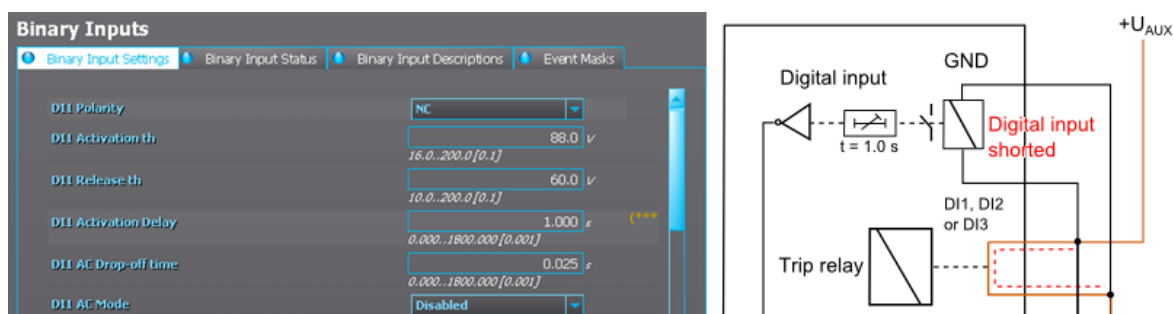
Figure. 7.3 - 204. Settings for a digital input used for trip circuit supervision.
