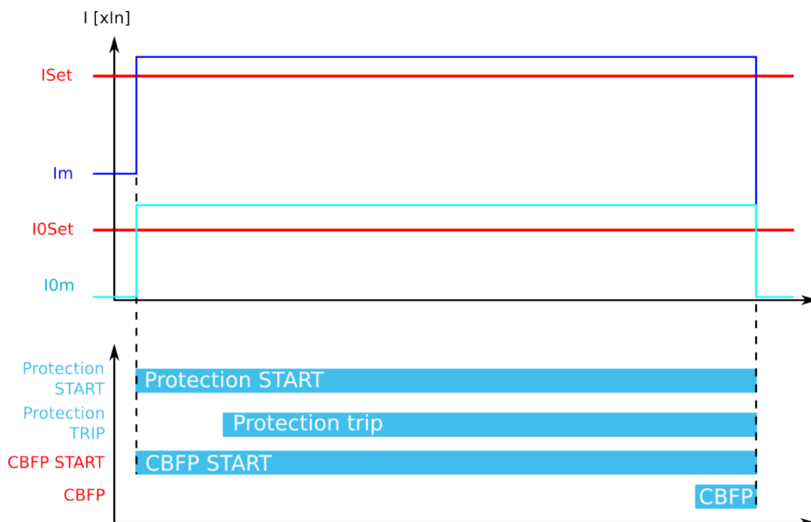
Figure. 5.4.8 - 51. CBFP when "Current" is the selected criterion.
