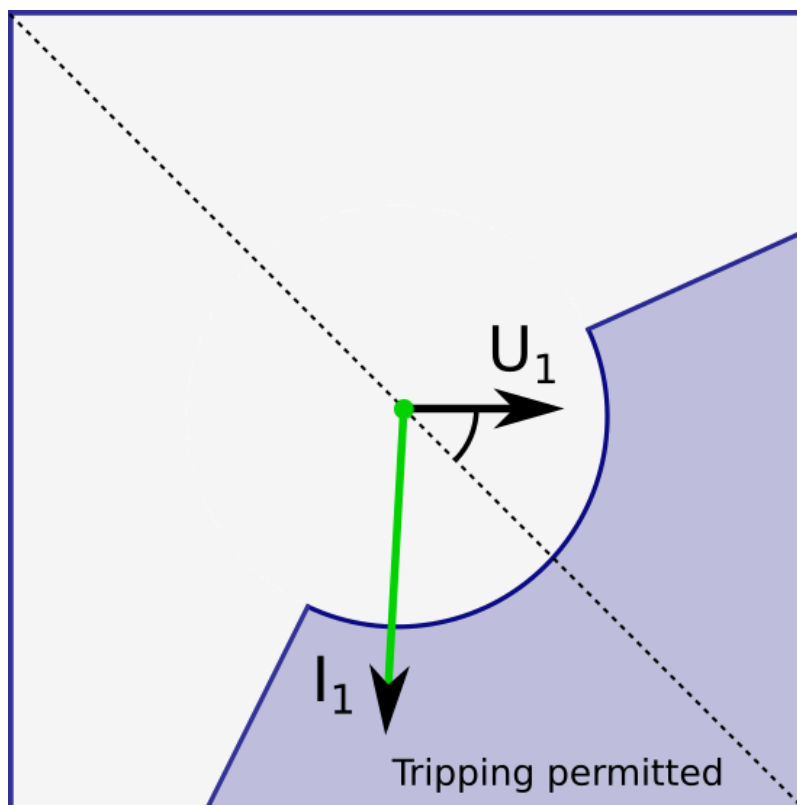
Figure. 5.4.4 - 34. Operation sector area when the sector center has been set to -45 degrees.
