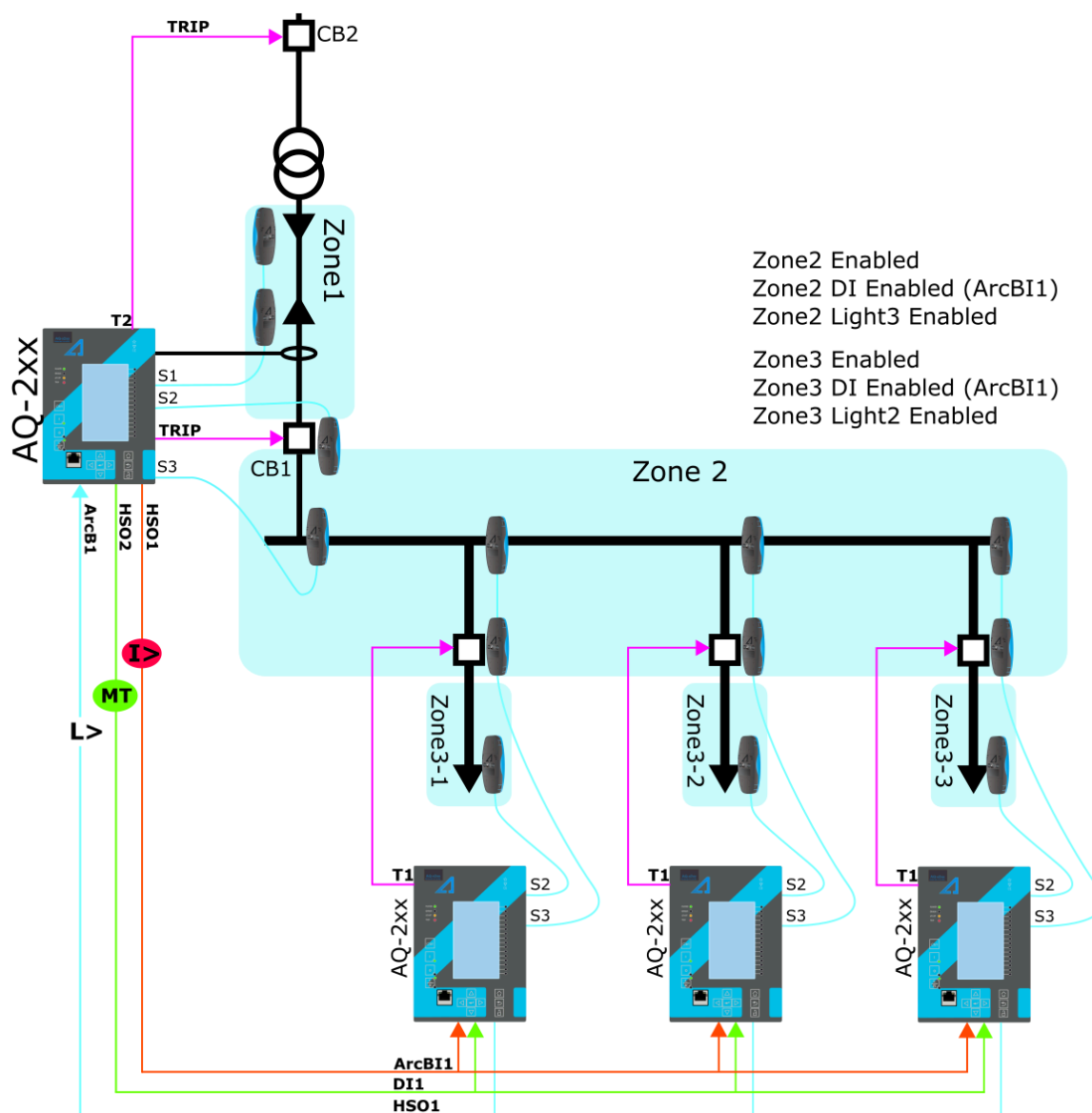
Figure. 5.4.23 - 133. Scheme IA1 (with AQ-200 protection relays).
