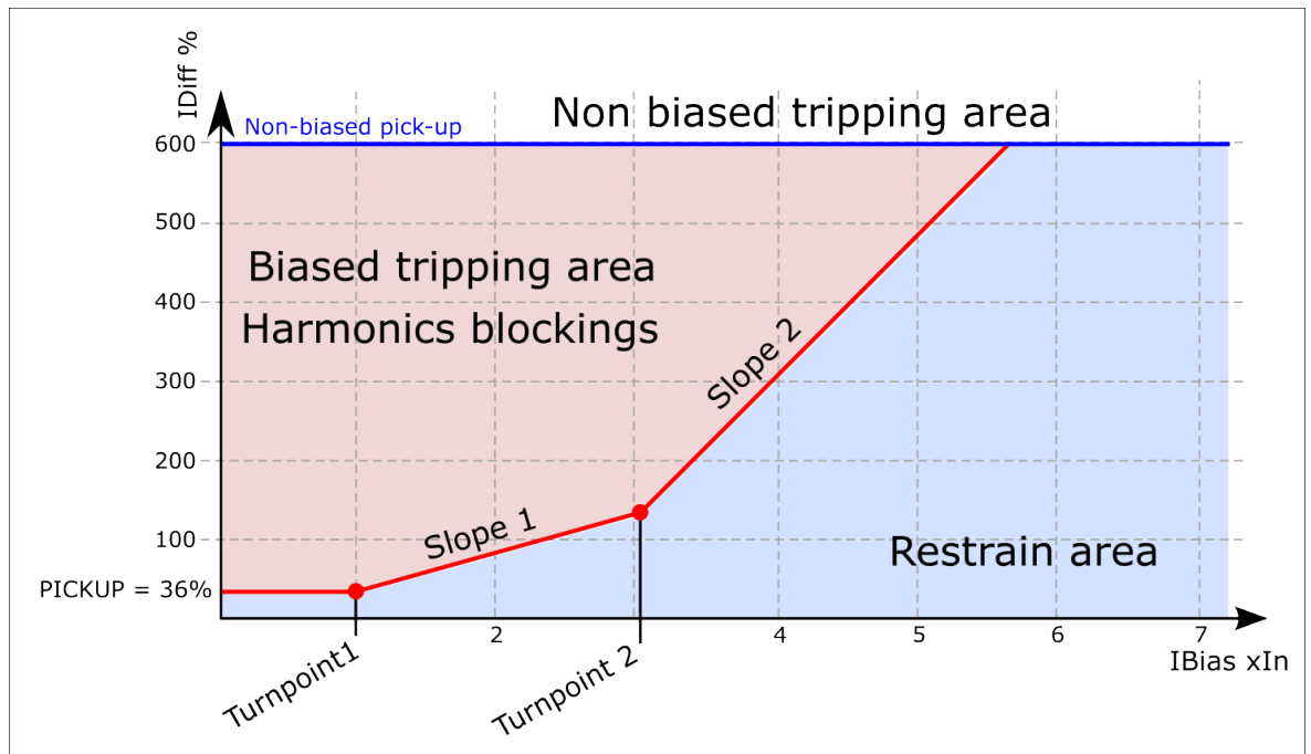
Figure. 5.4.21 - 115. Differential function characteristic, biased and non-biased.
