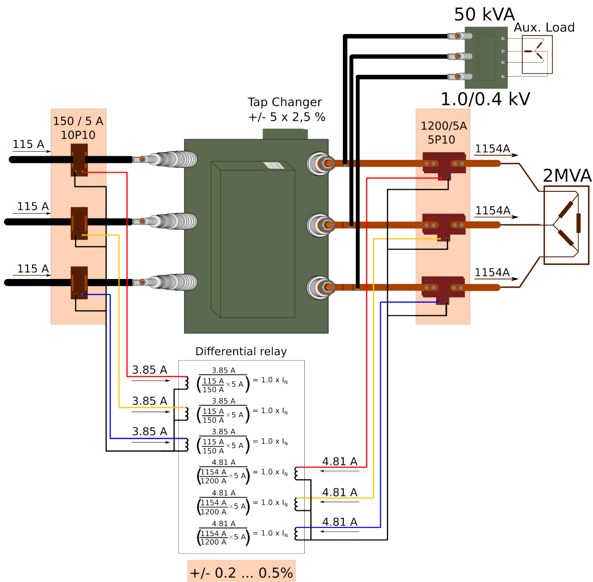
Figure. 5.4.21 - 116. Differential current sources (normal operation).
