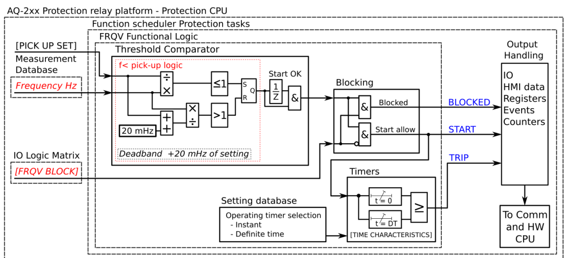
Figure. 5.4.14 - 87. Simplified function block diagram of the f < function.
