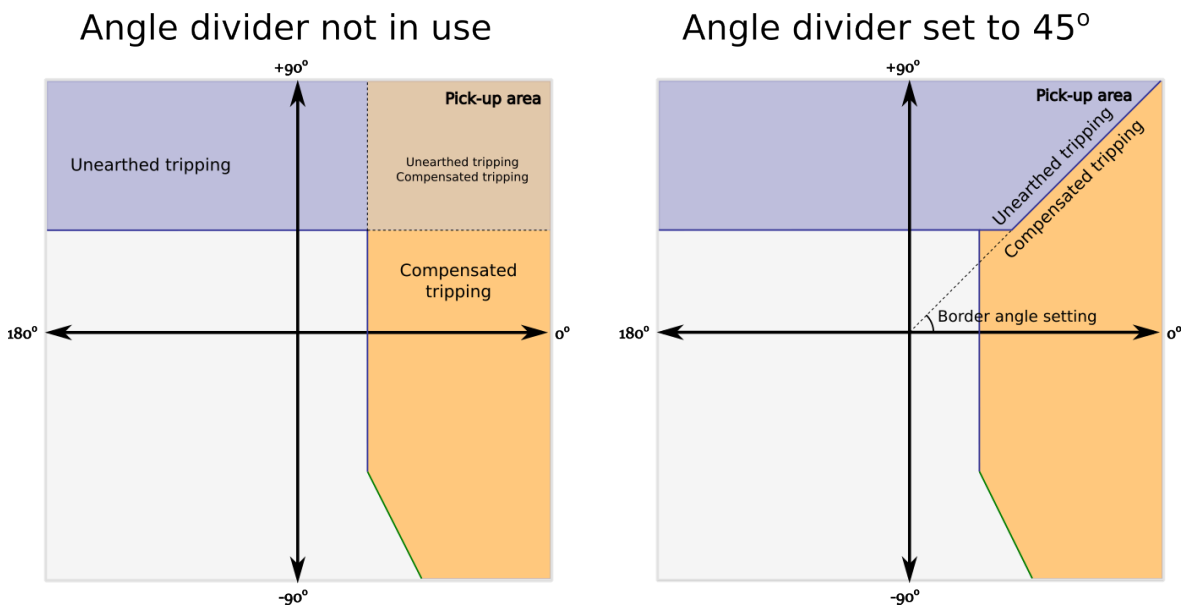
Figure. 5.4.5 - 41. Effect of angle divider when in use and when disabled.
