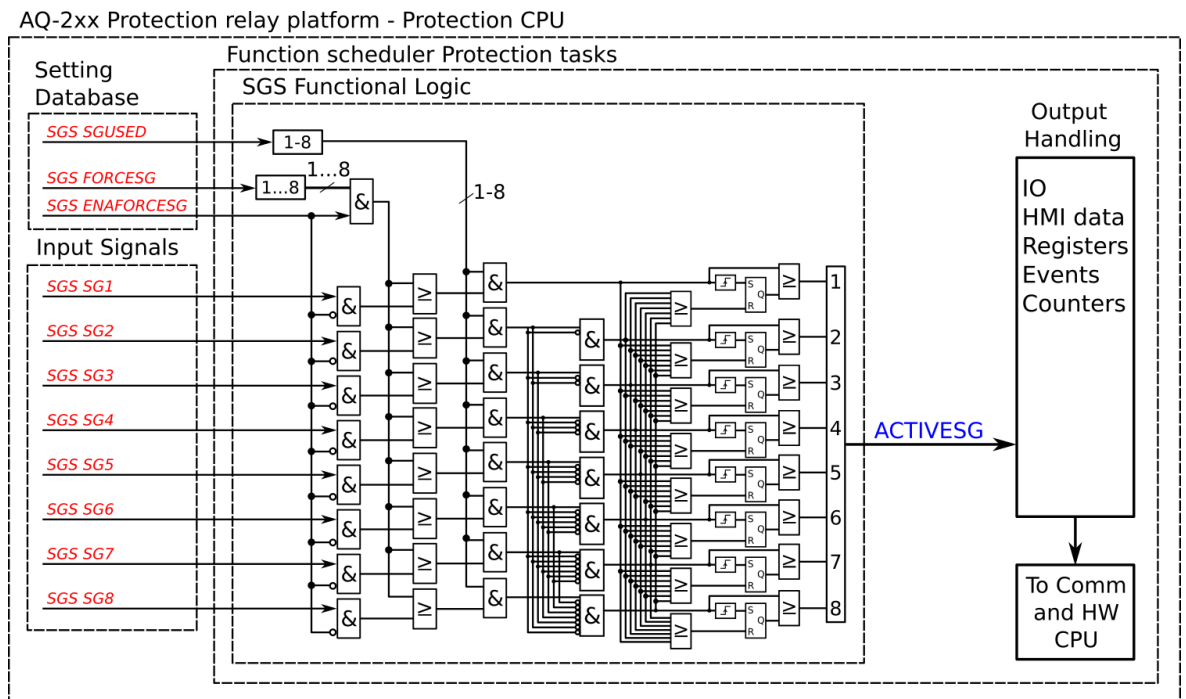
Figure. 5.5.3 - 154. Simplified function block diagram of the setting group selection function.
