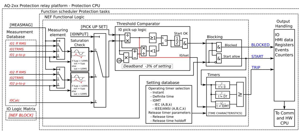
Figure. 5.4.3 - 31. Simplified function block diagram of the I0> function.
