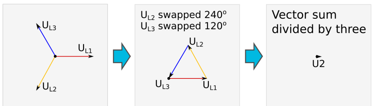
Figure. 5.4.13 - 81. Normal situation.
