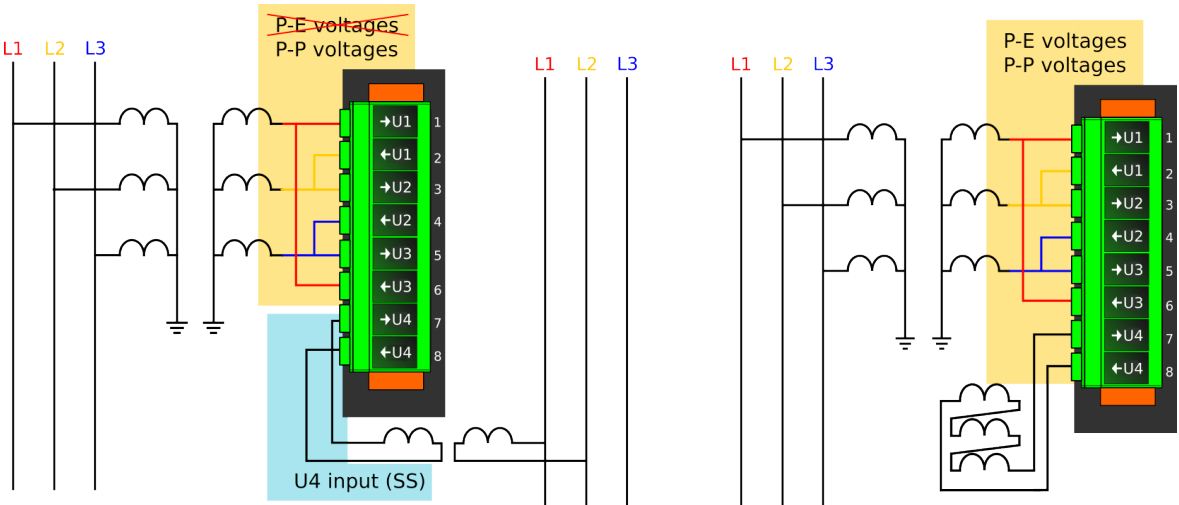
Figure. 5.4.11 - 71. Selectable measurement magnitudes with 3LL+U4 VT connection (P-E voltages not available without residual voltage).
