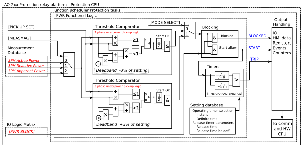
Figure. 5.4.16 - 91. Simplified function block diagram of the power protection function.
