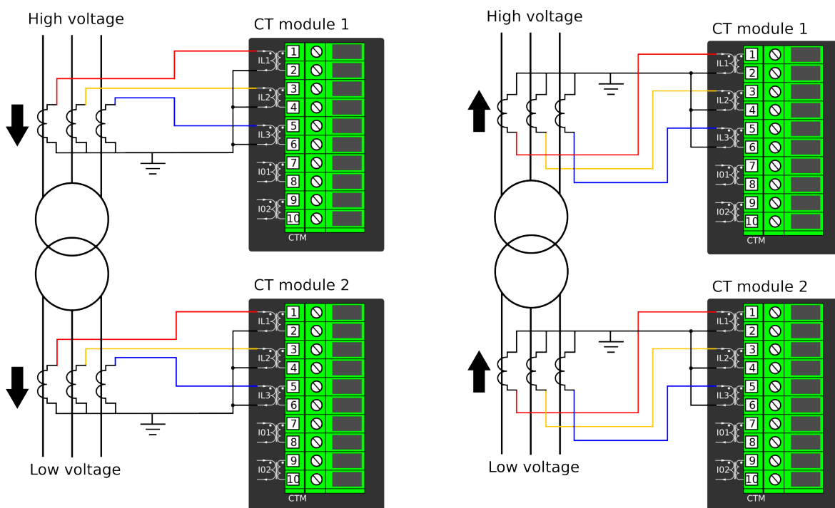
Figure. 5.4.21 - 112. CTs' starpoints requiring the "Subtract" mode.
