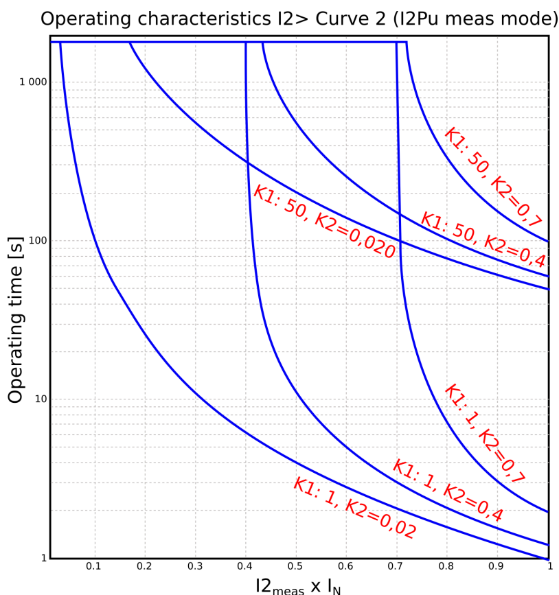
Figure. 5.4.4 - 22. Operation characteristics curve for I_2 > Curve2.
