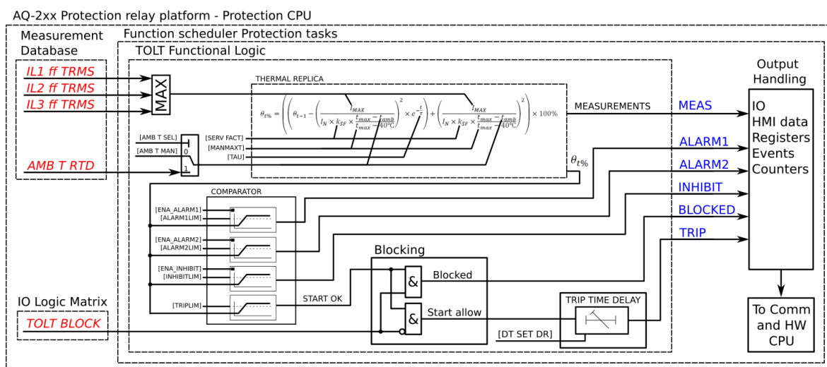
Figure. 5.4.9 - 48. Simplified function block diagram of the TT> function.
