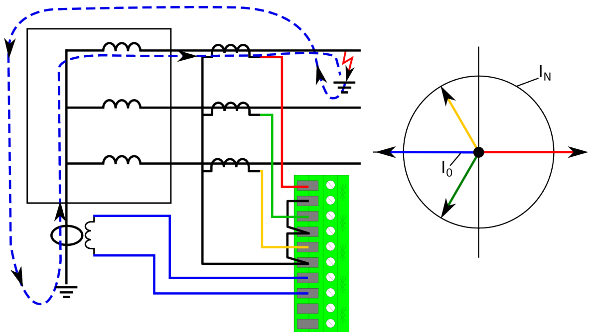
Figure. 5.4.7 - 42. Restricted earth fault outside a Y winding transformer.
