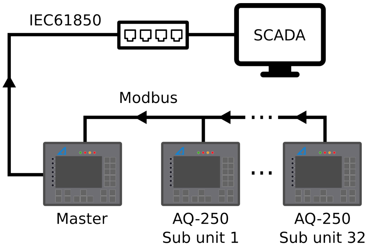
Figure. 6.4 - 110. Example setup of Modbus Gateway application.
