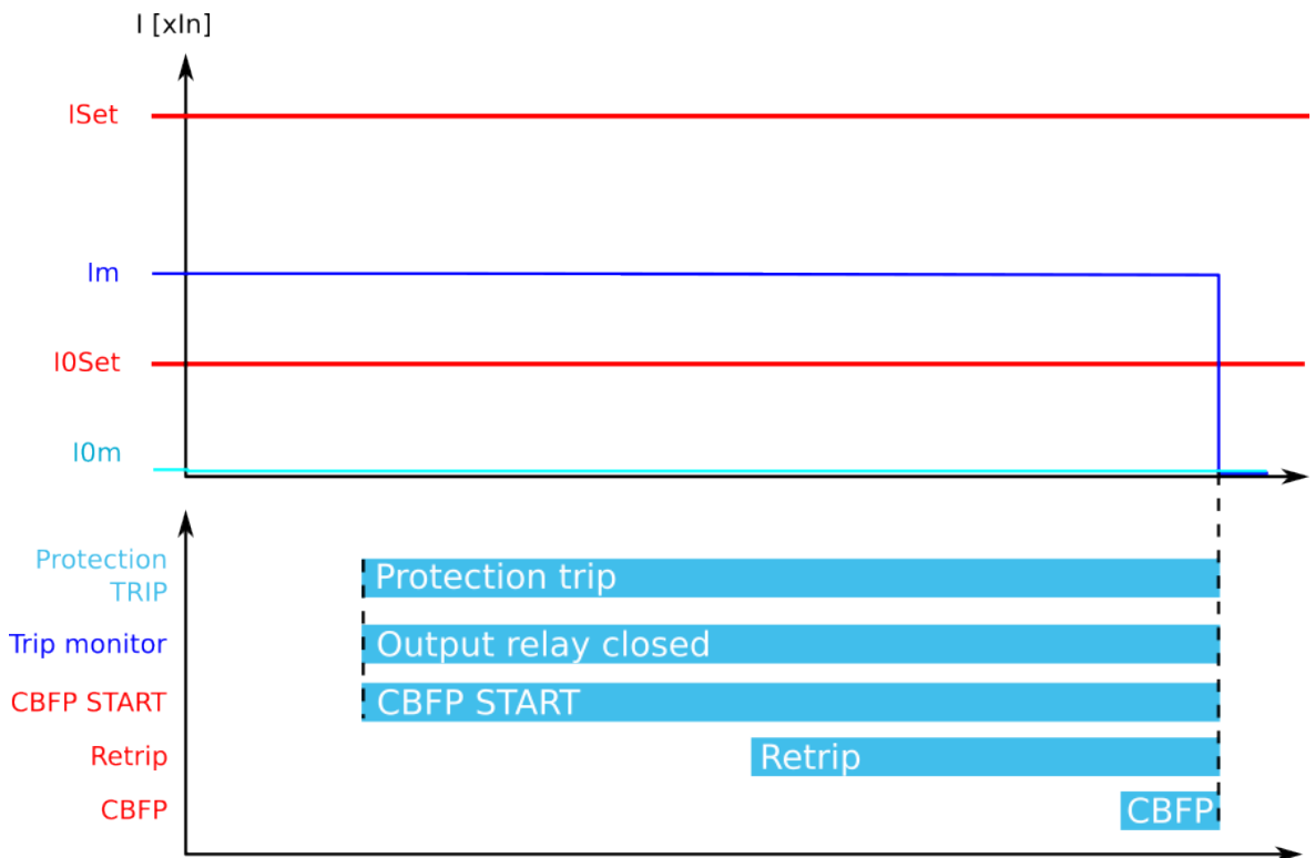
Figure. 5.4.6 - 28. Retrip and CBFP when "Current or DO" is the selected criterion.
