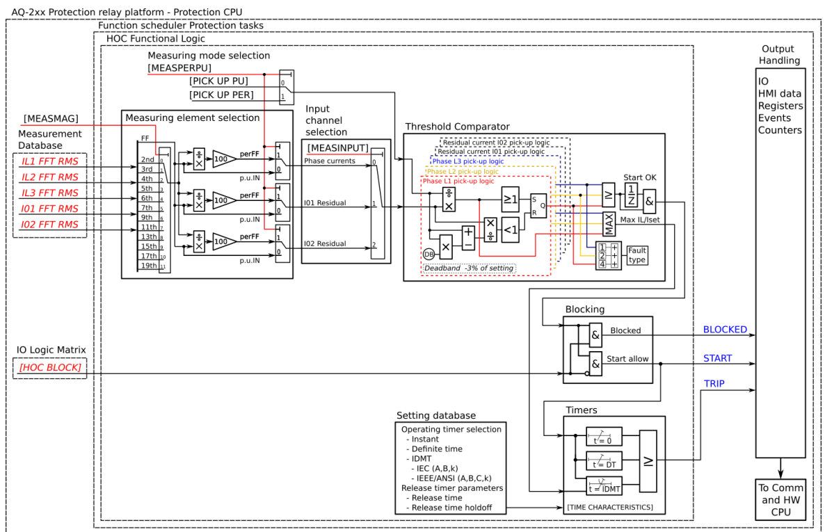
Figure. 5.4.5 - 23. Simplified function block diagram of the Ih> function.
