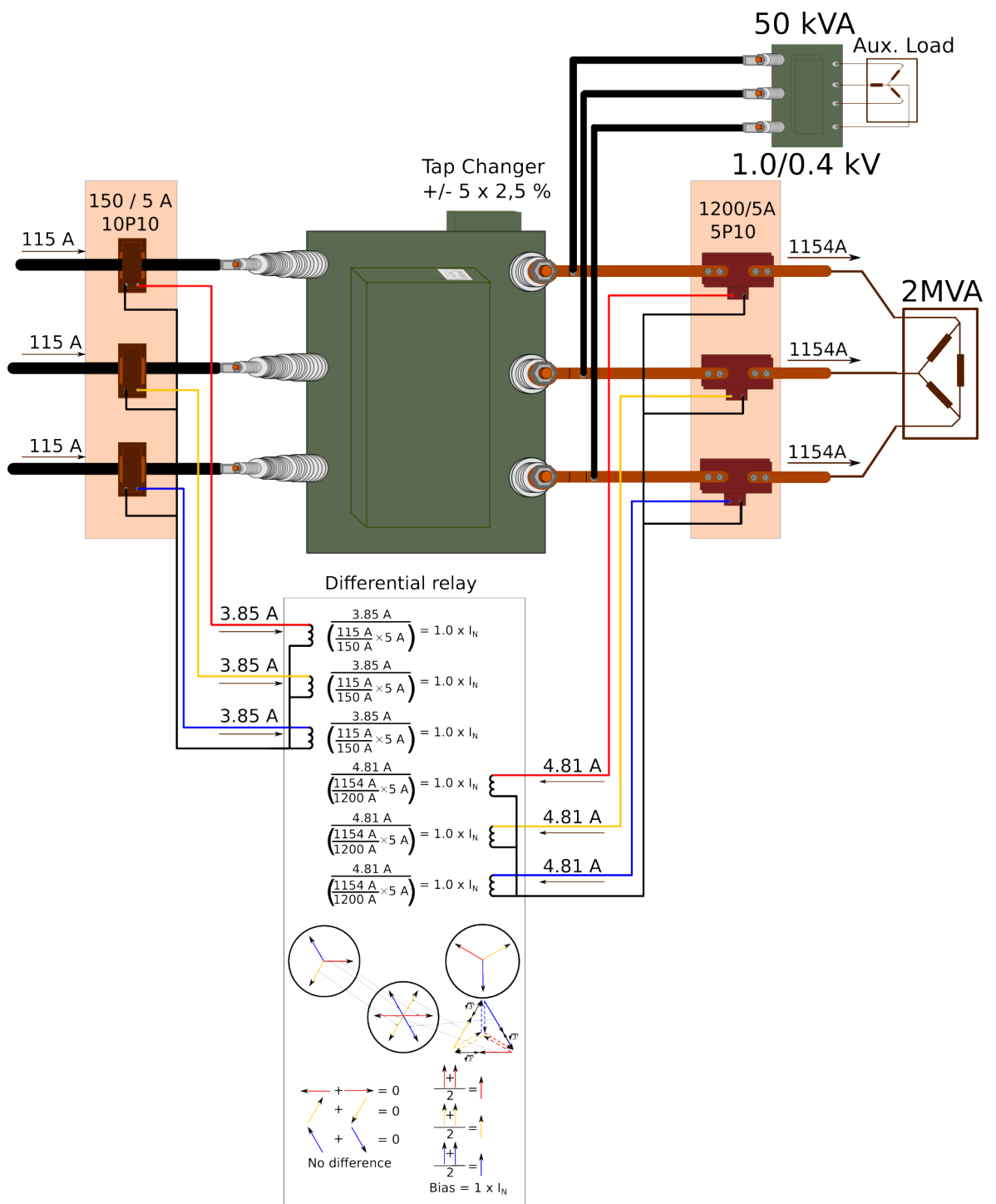
Figure. 5.4.10 - 112. Example configuration for the transformer differential function.
