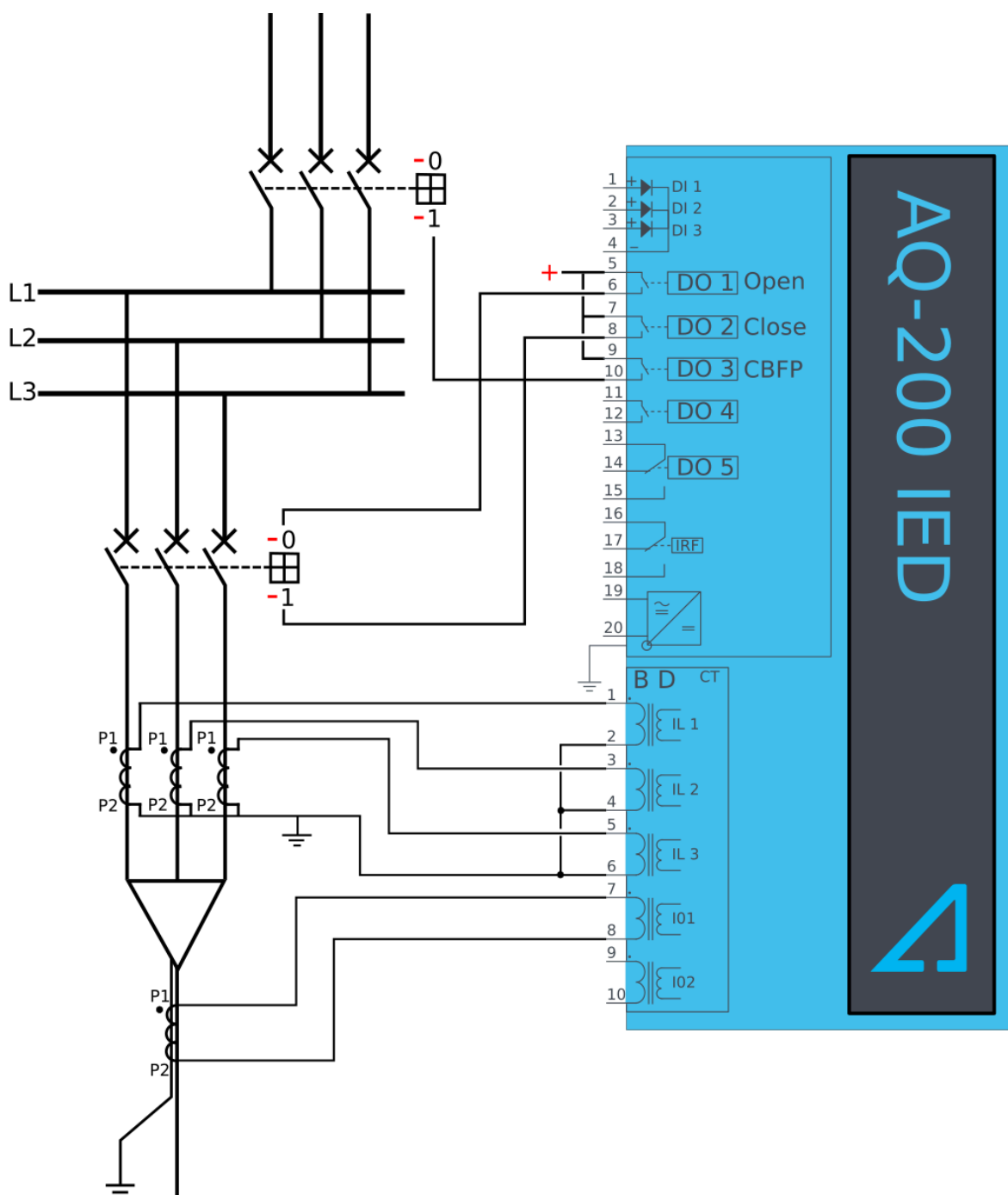
Figure. 5.4.6 - 77. Wiring diagram when Trip and CBFP are configured to the device.
