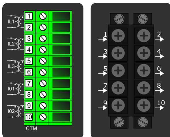
Figure. 8.3 - 171. Module connections with standard and ring lug terminals.
