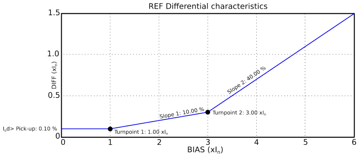
Figure. 5.4.7 - 84. Differential characteristics for the I0d> function with default settings.
