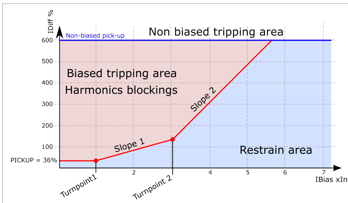
Figure. 5.4.10 - 109. Differential function characteristic, biased and non-biased.
