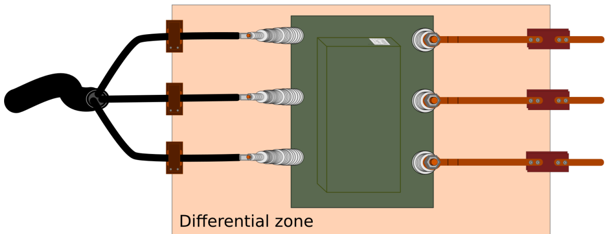
Figure. 5.4.10 - 98. Transformer and its components forming the differential zone.
