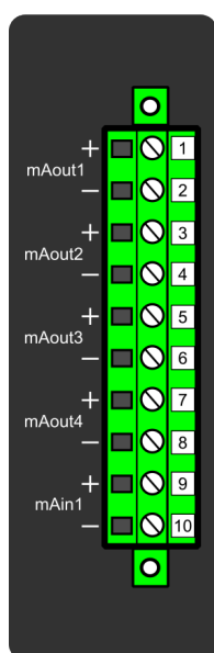
Figure. 8.12 - 185. Milliampere (mA) I/O module connections.
