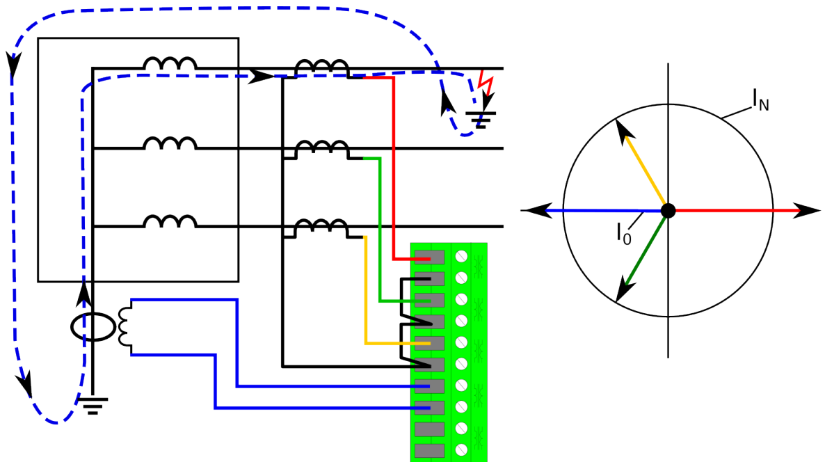
Figure. 5.4.7 - 90. Restricted earth fault outside a Y winding transformer.
