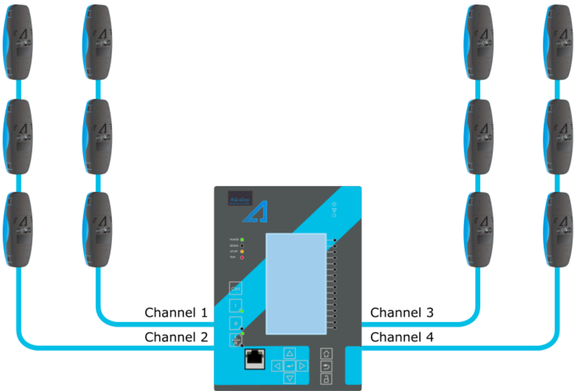
Figure. 5.4.12 - 125. IED equipped with arc protection.
