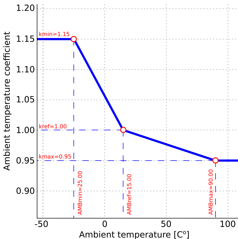
Figure. 5.4.9 - 95. Ambient temperature coefficient calculation (a three-point linear approximation and a settable correction curve).
