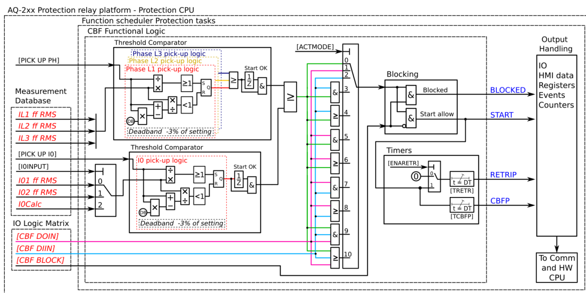
Figure. 5.4.6 - 72. Simplified function block diagram of the CBFP function.
