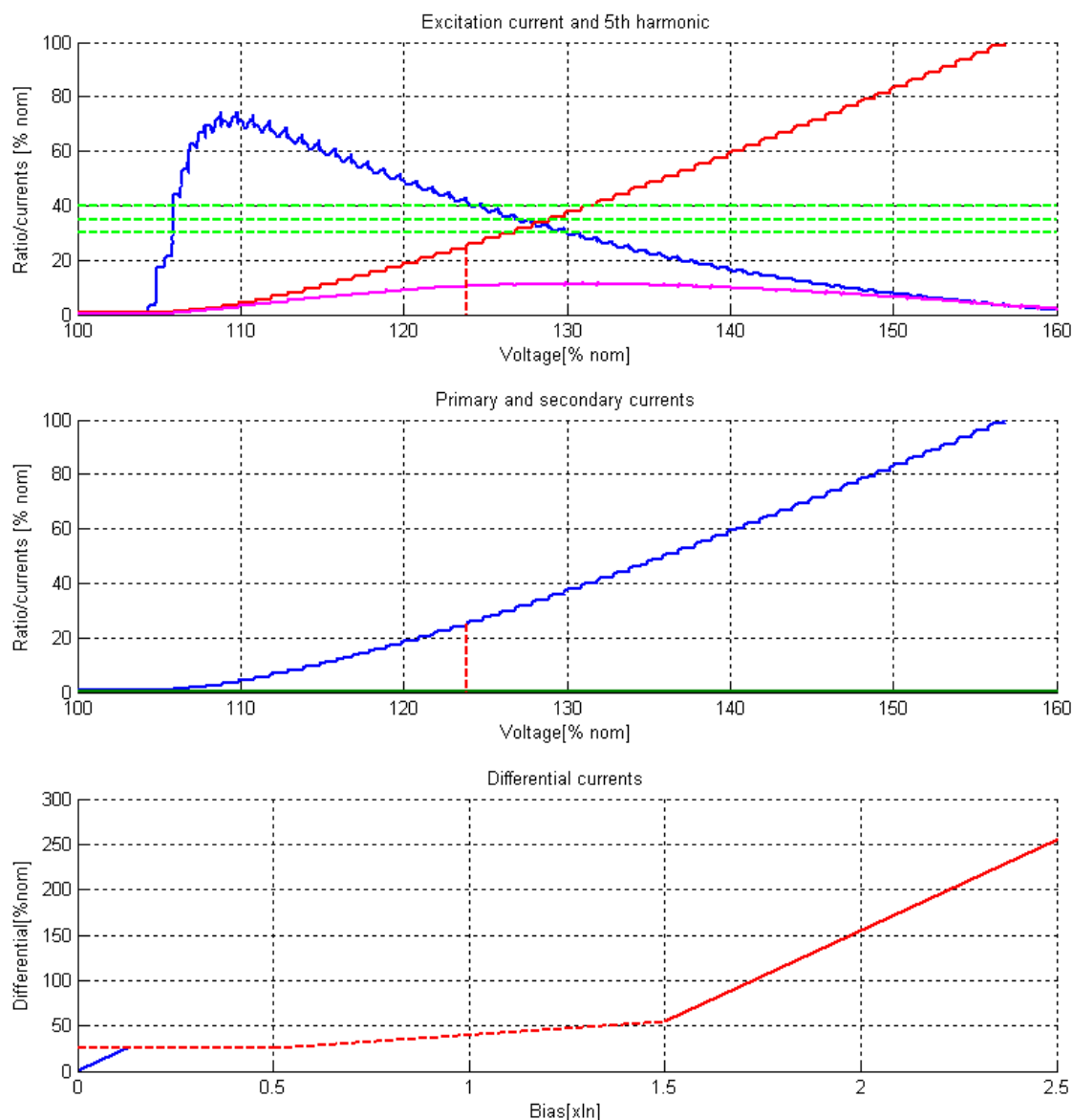
Figure. 5.4.10 - 120. Transformer behavior in case of overvoltage caused by overexcitation.
