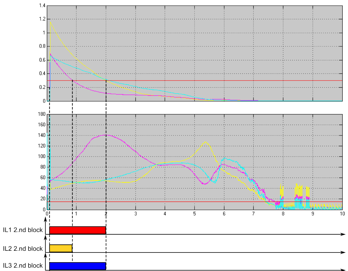
Figure. 5.4.10 - 119. Example of transformer magnetizing inrush currents.
