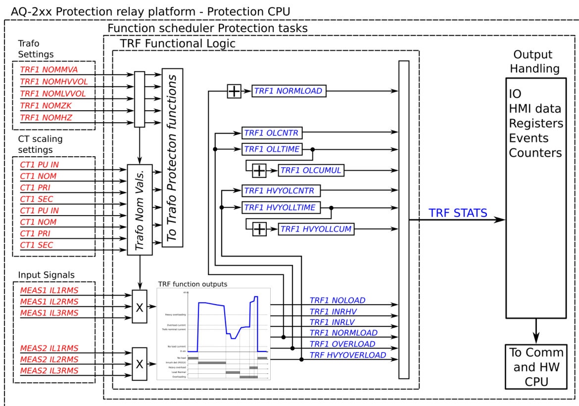
Figure. 5.4.8 - 92. Simplified function block diagram of the transformer status monitoring function.
