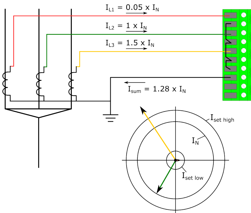
Figure. 5.6.1 - 145. No wiring fault but heavy unbalance.
