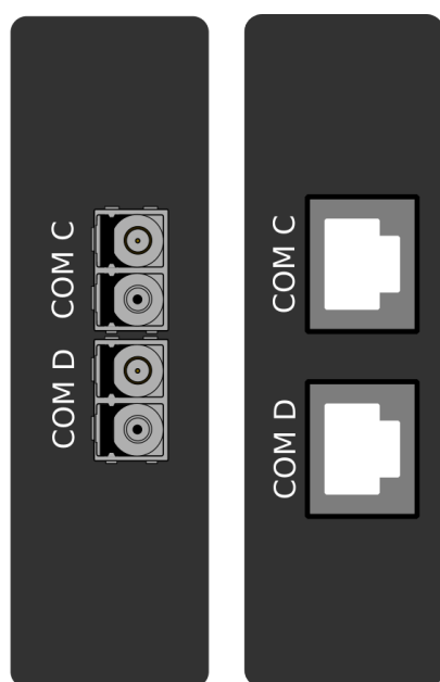
Figure. 8.9 - 179. LC and RJ45 100 Mbps Ethernet module connectors.
