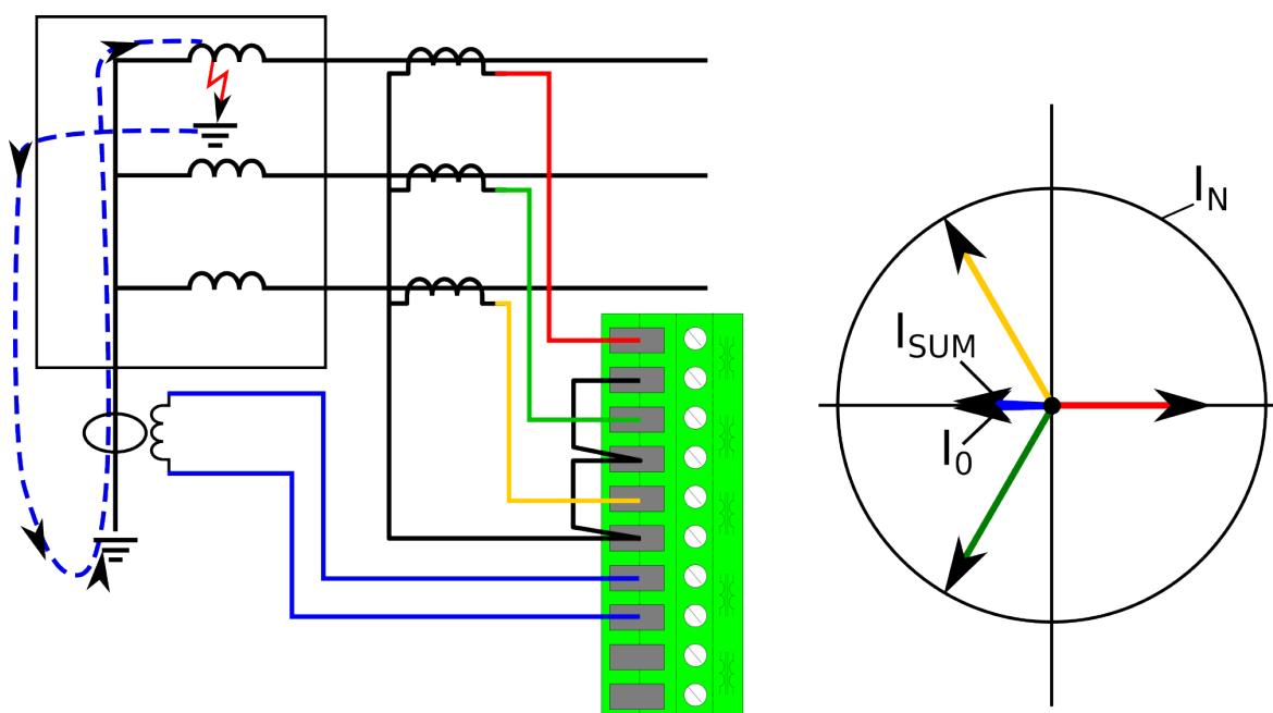
Figure. 5.4.7 - 91. Restricted earth fault inside a Y winding transformer.
