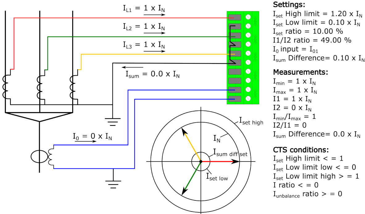
Figure. 5.6.1 - 147. Normal situation, residual current also measured.
