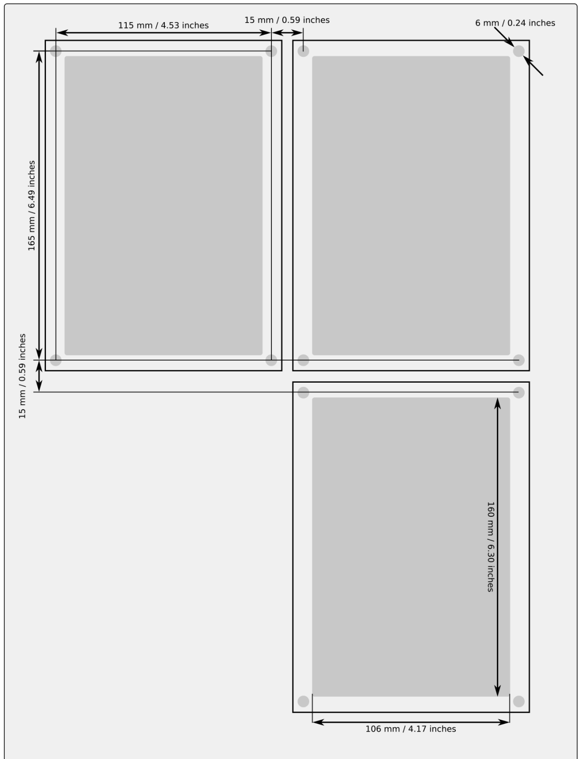
Figure. 8.13 - 188. Panel cutout dimensions and device spacing.
