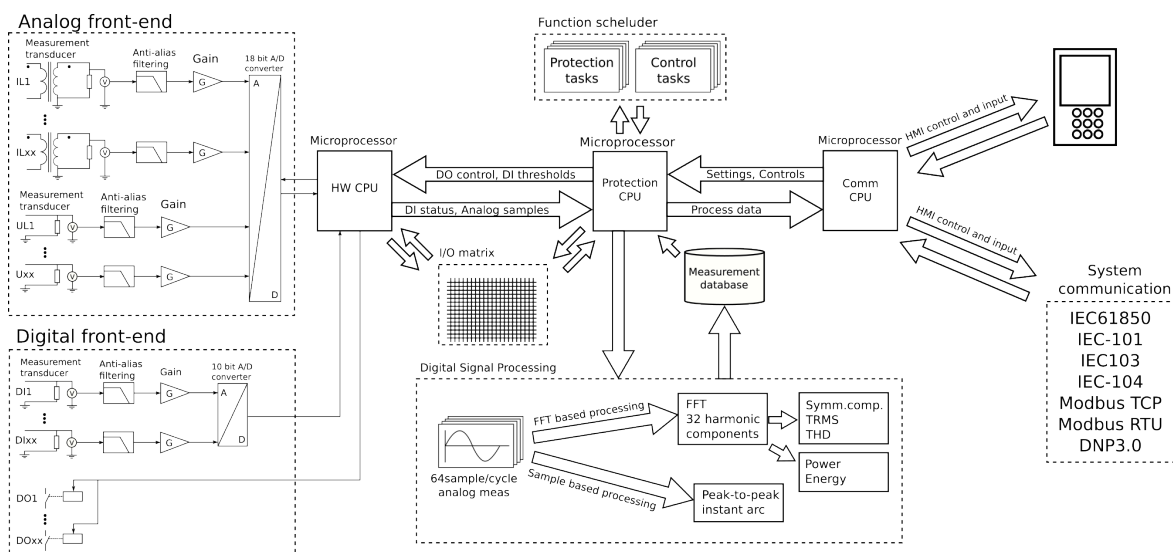
Figure. 5.4.1 - 58. Principle diagram of the protection relay platform.
