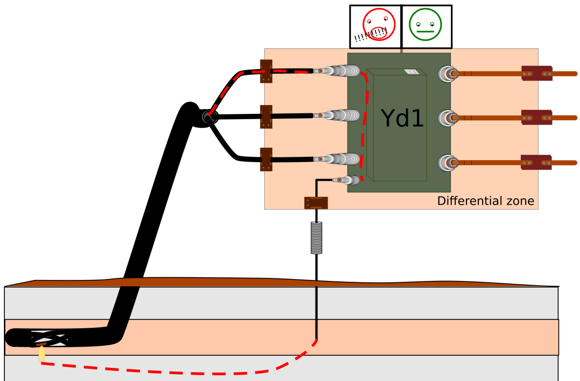
Figure. 5.4.10 - 114. Transformer earthing settings that do not compensate for external earth faults.
