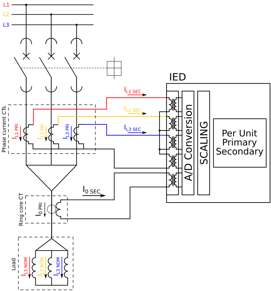
Figure. 5.2.1 - 51. Current measurement terminology
