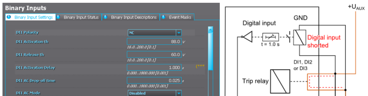
Figure. 7.3 - 164. Settings for a digital input used for trip circuit supervision.
