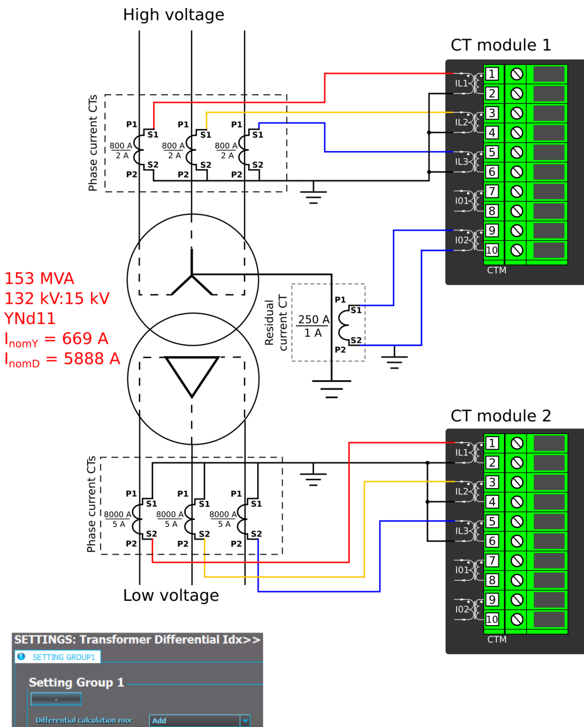
Figure. 5.2.1 - 57. Connections (application 2).
