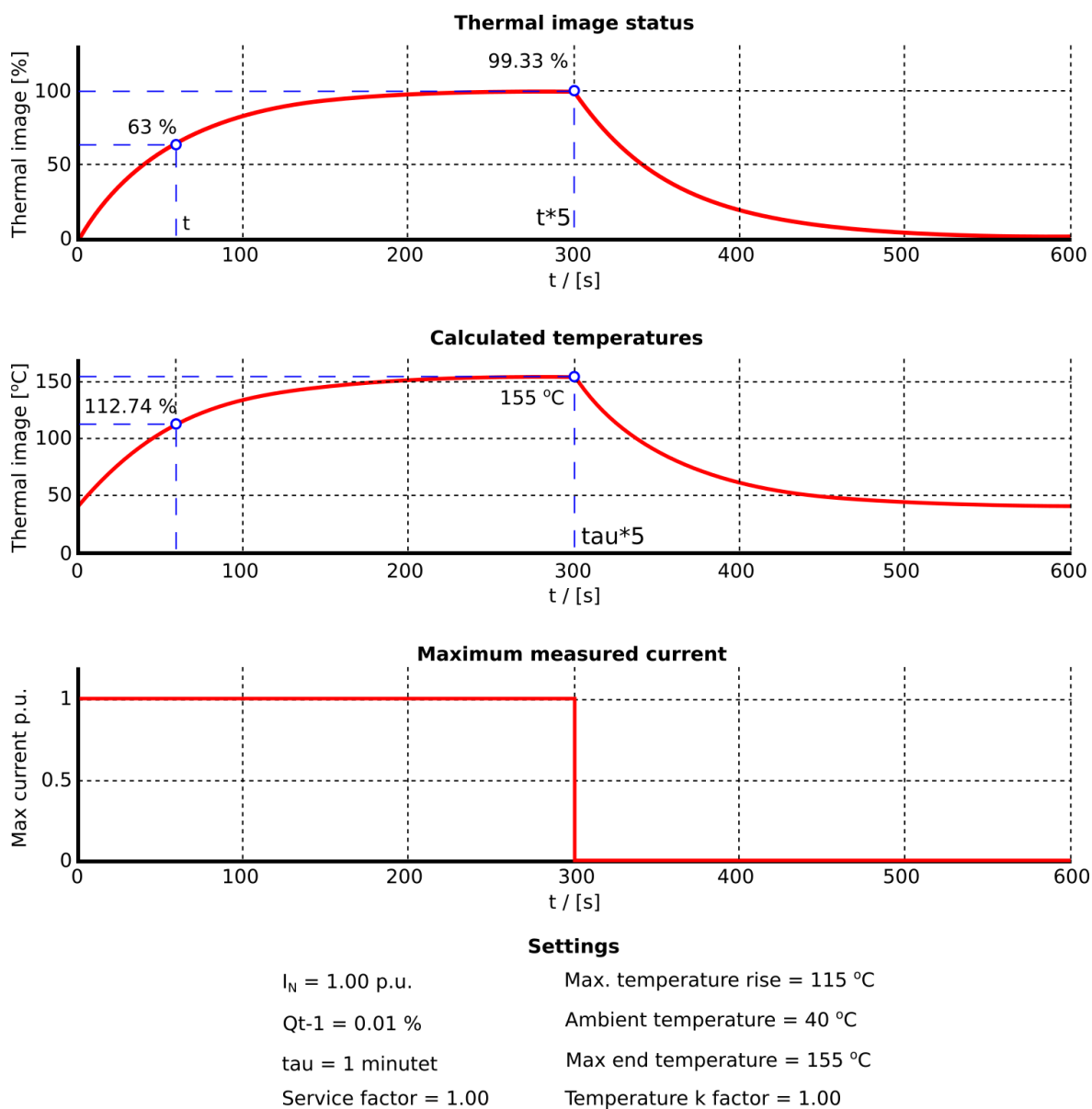
Figure. 5.4.9 - 94. Example of thermal image calculation with nominal conditions.
