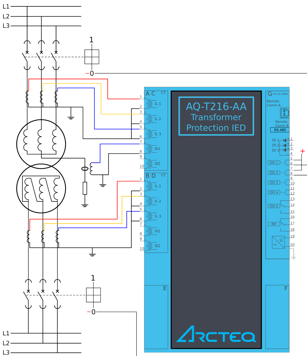
Figure. 7.2 - 162. Application example and its connections.
