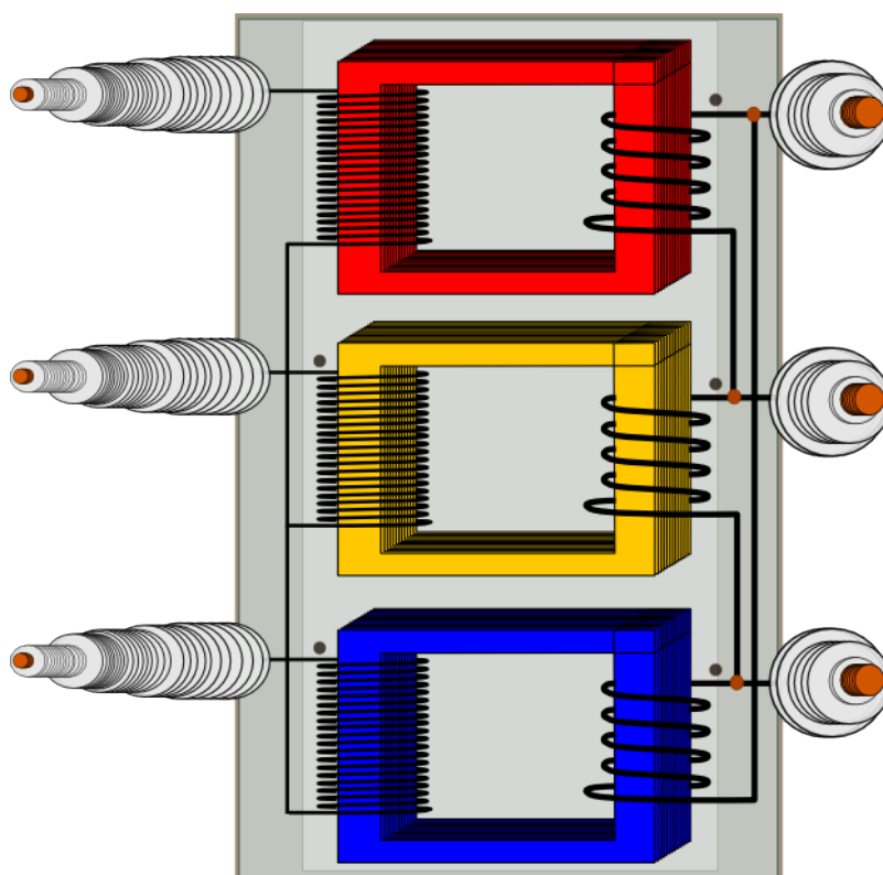
Figure. 5.4.10 - 101. Yd1 transformer's internal connection (in theory).
