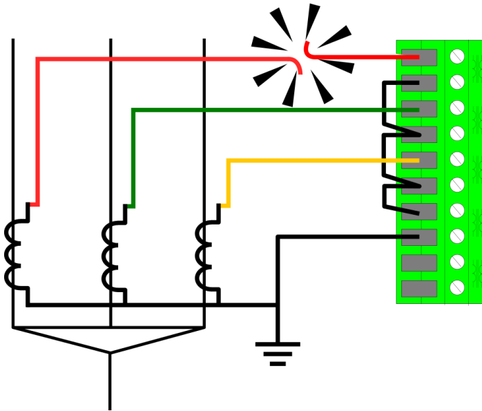
Figure. 5.6.1 - 140. Secondary circuit fault in phase L1 wiring.
