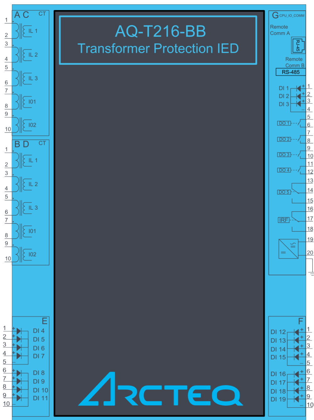
Figure. 7.1 - 160. AQ-T216 variant with digital input modules.
