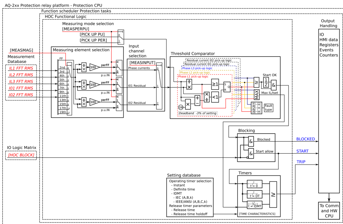
Figure. 5.4.5 - 71. Simplified function block diagram of the lh> function.
