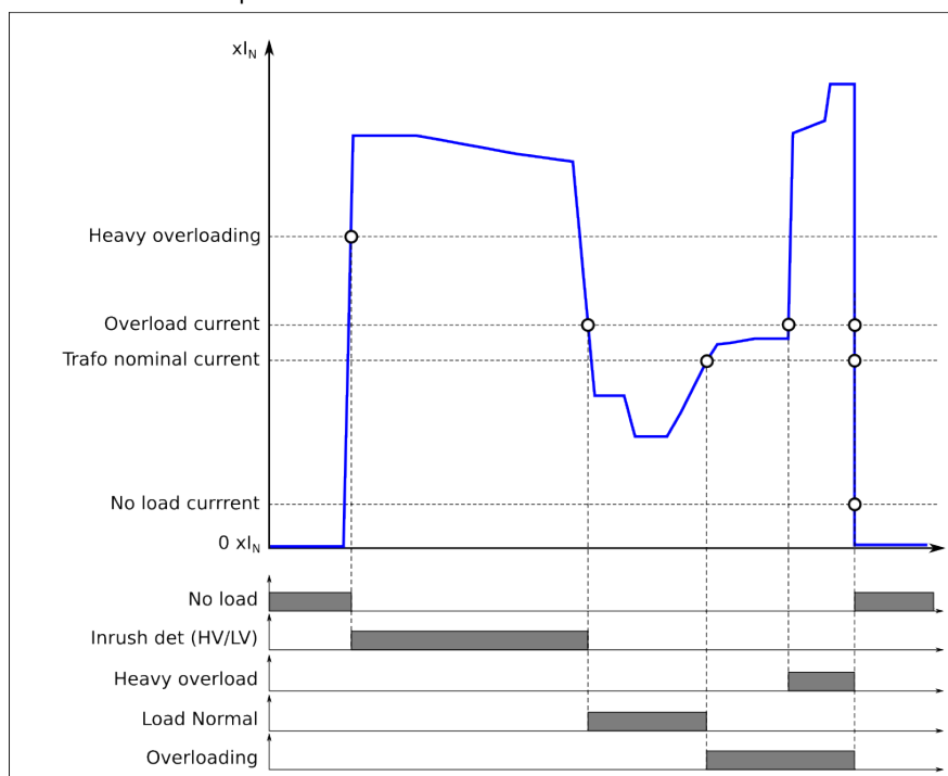
Figure. 5.4.8 - 93. Activation of the function's outputs.
