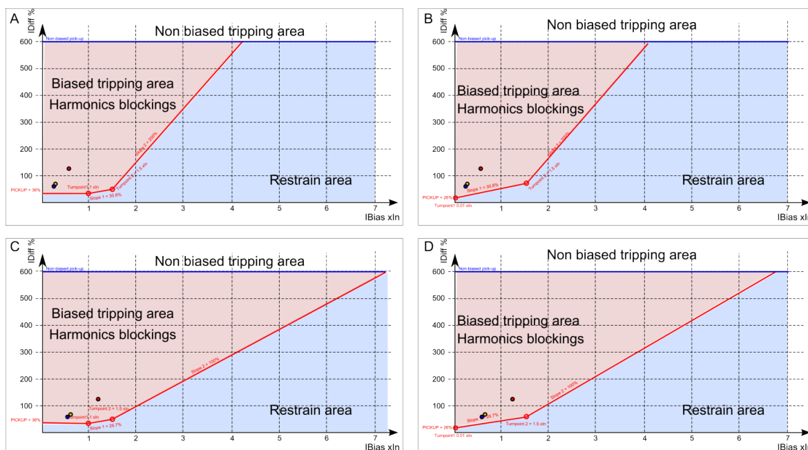
Figure. 5.4.10 - 117. Differential currents in the energization of a 2 MVA transformer.
