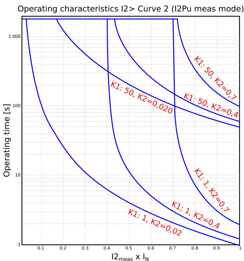
Figure. 5.4.4 - 70. Operation characteristics curve for I_2 > Curve2.
