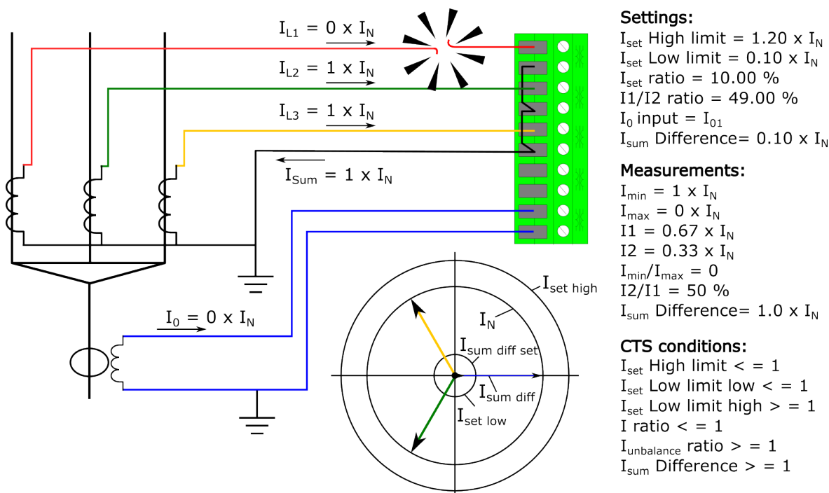
Figure. 5.6.1 - 148. Broken secondary phase current wiring.
