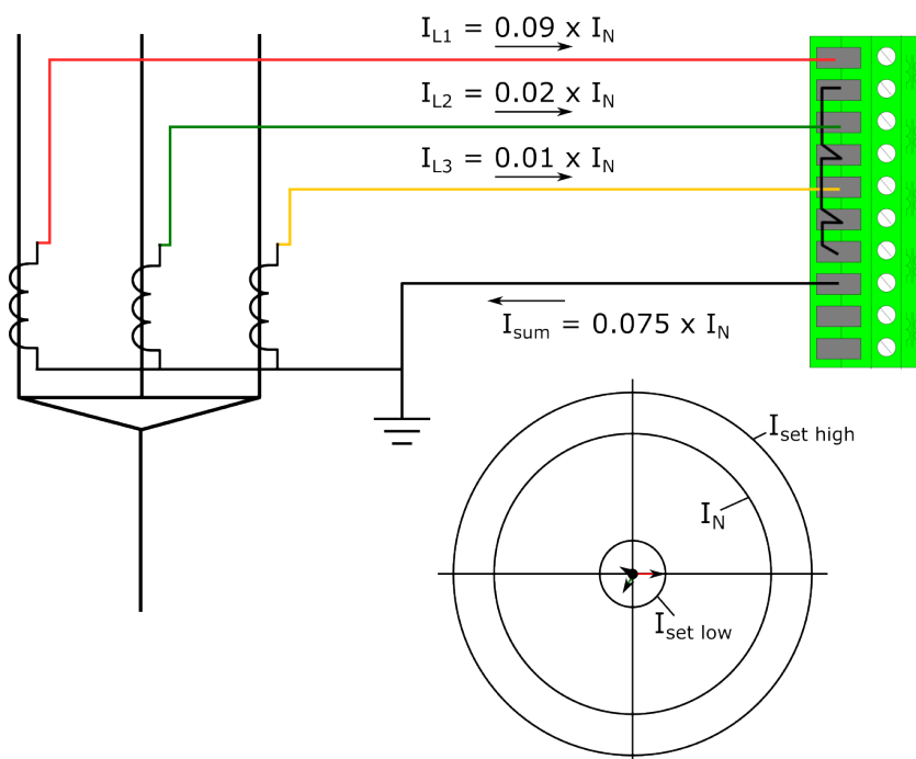
Figure. 5.6.1 - 146. Low current and heavy unbalance.
