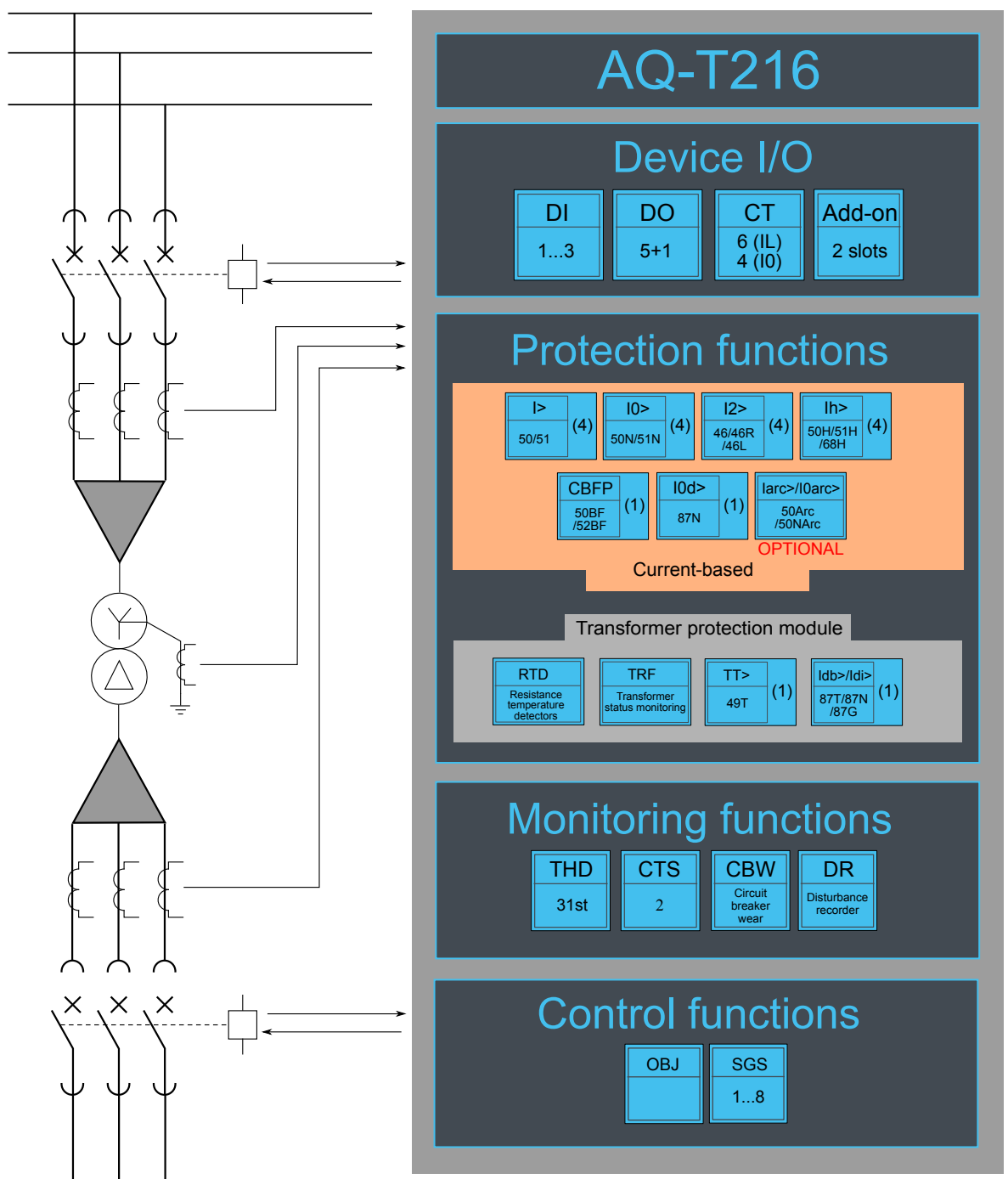
Figure. 7.1 - 161. AQ-T216 application example with function block diagram.
