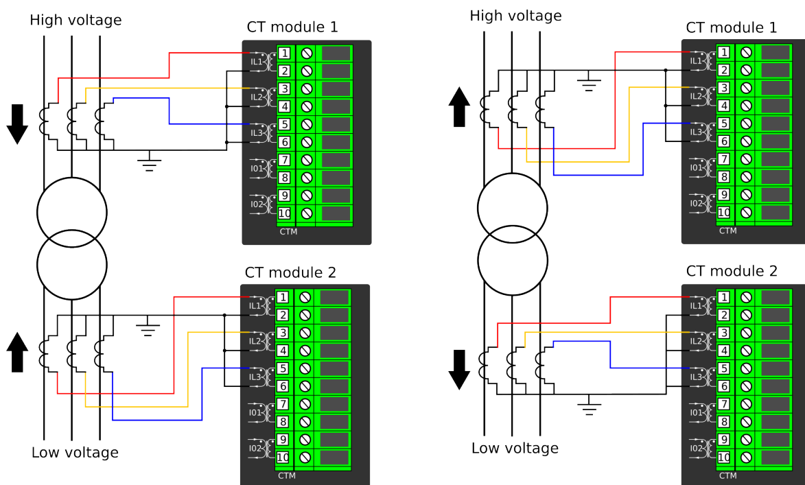
Figure. 5.4.10 - 105. CTs' starpoints requiring the "Add" mode.
