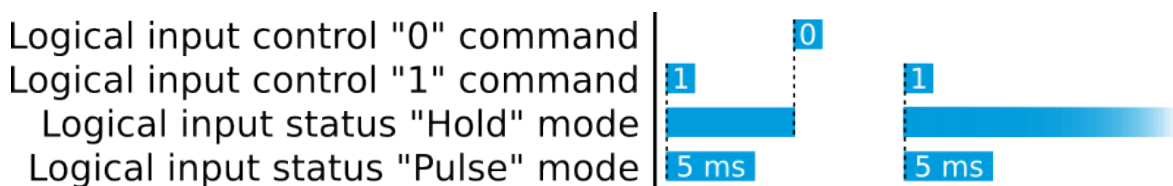
Figure. 5.5.9 - 138. Operation of logical input in "Hold" and "Pulse" modes.
