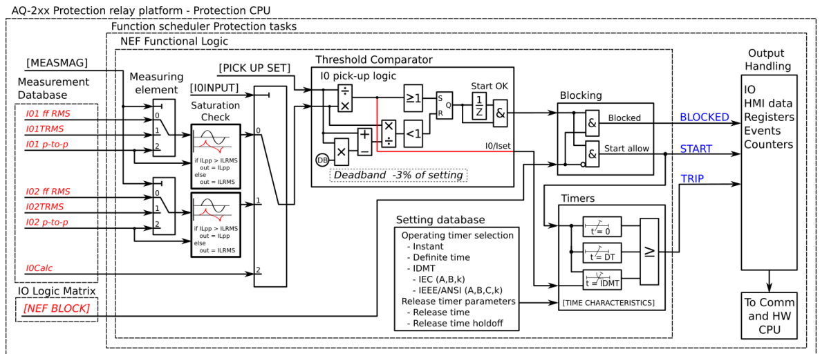
Figure. 5.4.3 - 68. Simplified function block diagram of the I0> function.
