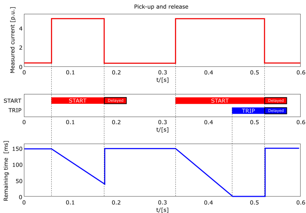
Figure. 5.4.1 - 65. Delayed pick-up release, delay counter value is held during the release time.
