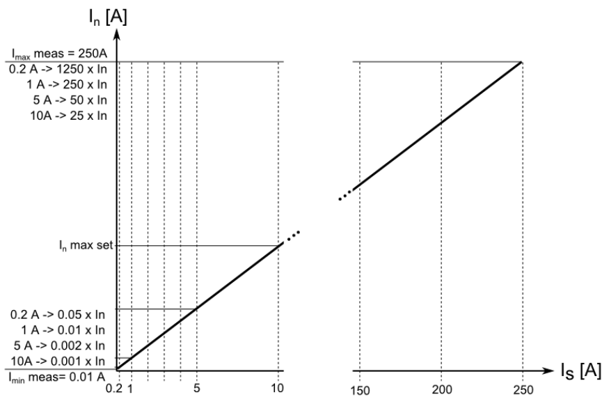
Figure. 5.4.1 - 60. Measurement range in relation to the nominal current.
