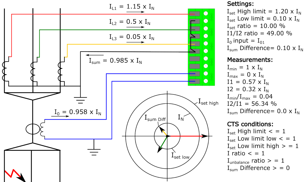
Figure. 5.6.1 - 150. Primary side high-impedance earth fault.
