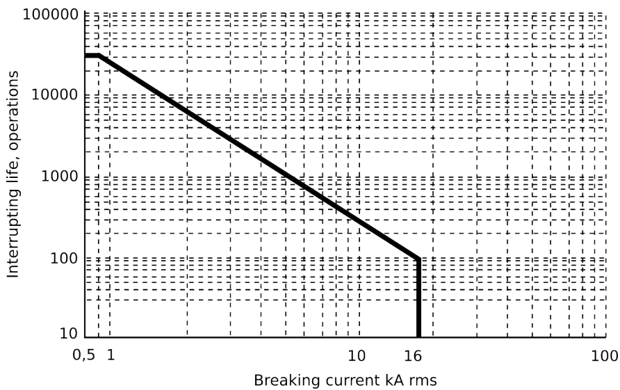
Figure. 5.6.2 - 151. Example of the circuit breaker interrupting life operations.
