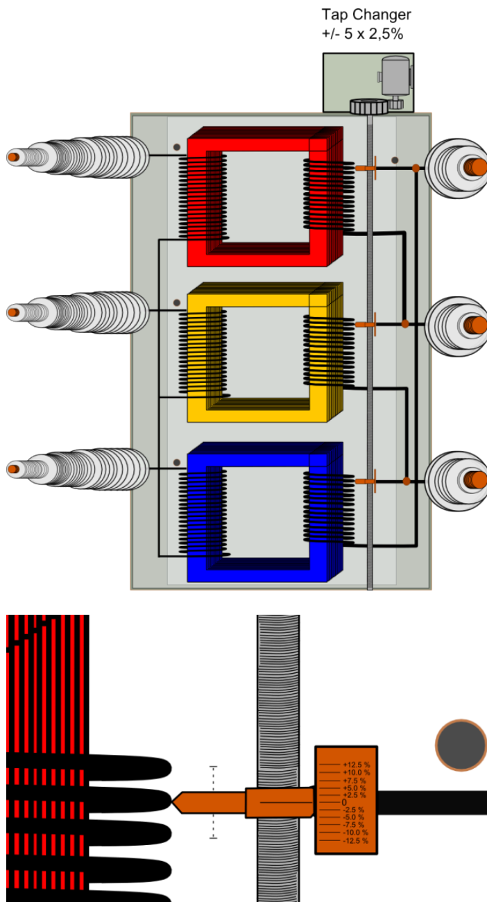
Figure. 5.4.10 - 111. Transformer tap changer.
