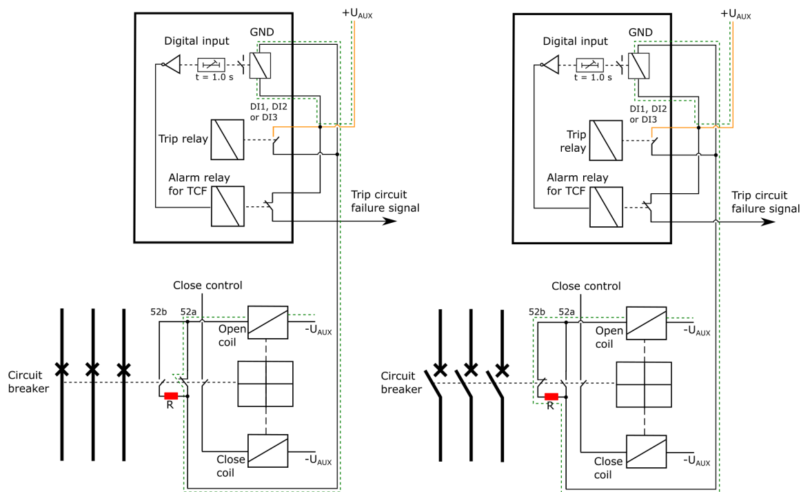
Figure. 7.3 - 163. Trip circuit supervision with one DI and one non-latched trip output.
