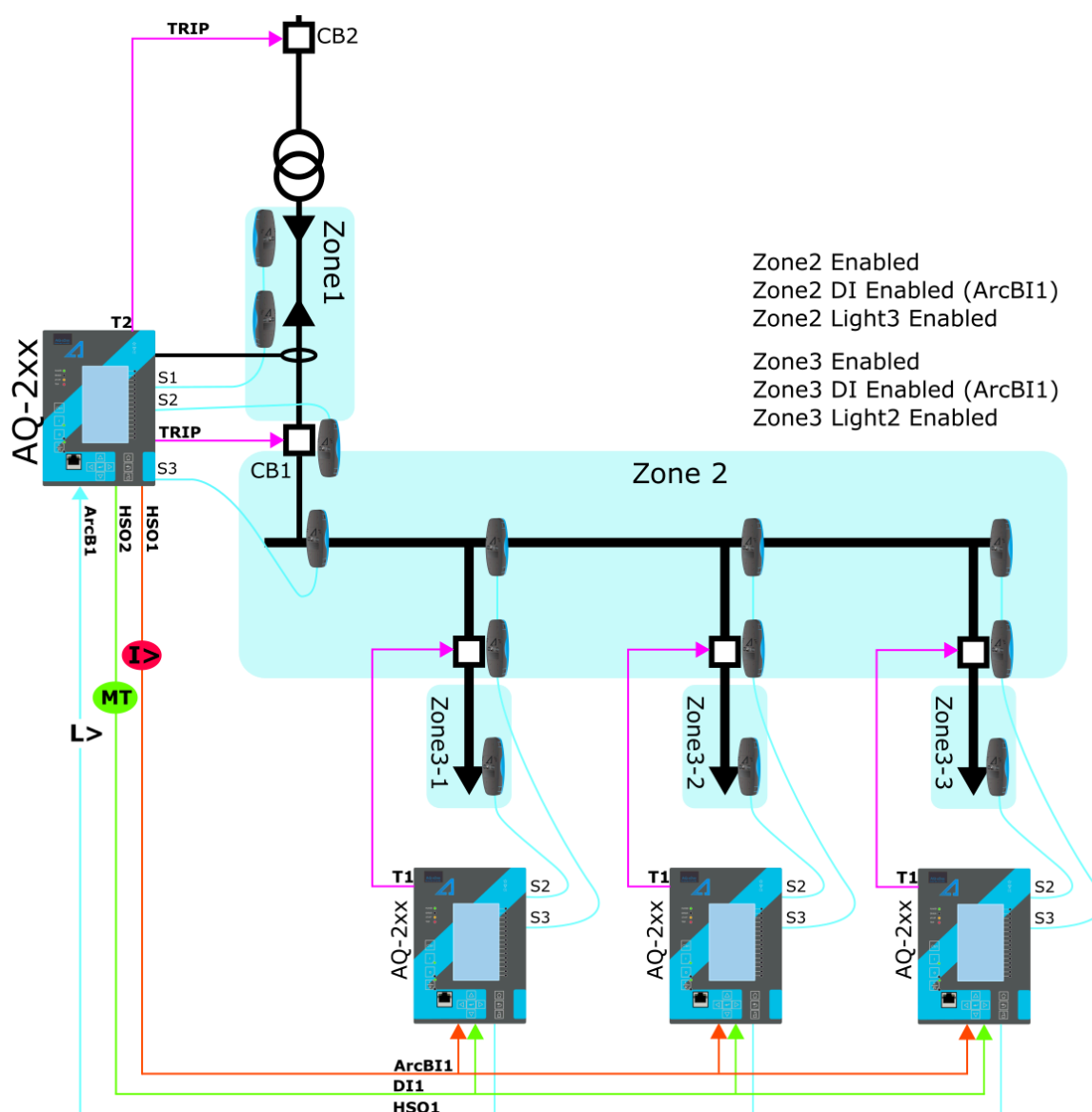
Figure. 5.4.12 - 127. Scheme IA1 (with AQ-200 protection relays).
