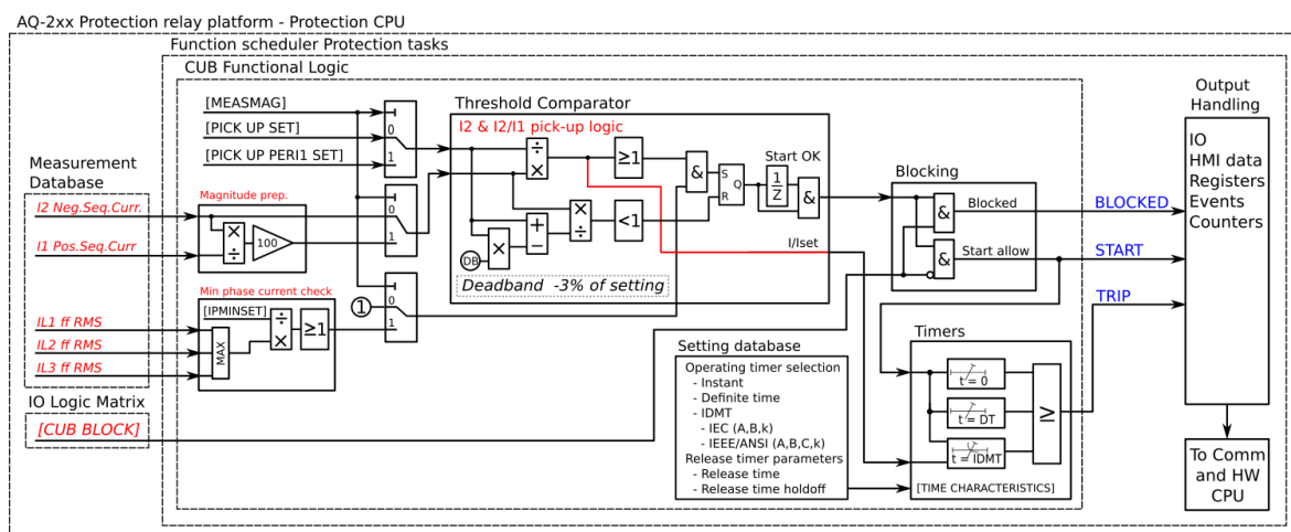
Figure. 5.4.4 - 69. Simplified function block diagram of the I2> function.
