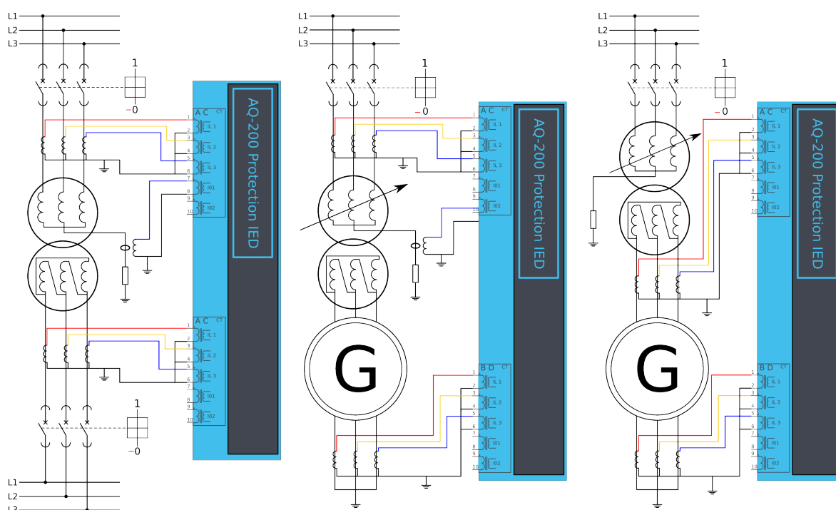
Figure. 5.4.10 - 97. Differential protection function can be used for protecting transformers, generators and both at the same time.
