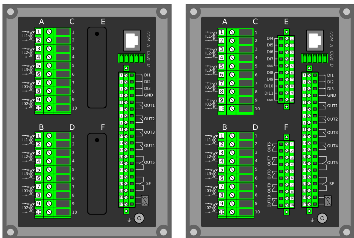
Figure. 8.1 - 168. Modular construction of AQ-X216.
