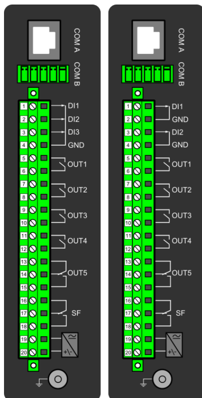
Figure. 8.2 - 170. CPU module.
