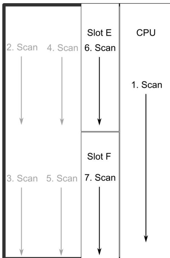
Figure. 8.1 - 169. AQ-X216 hardware scanning and I/O naming principles.
