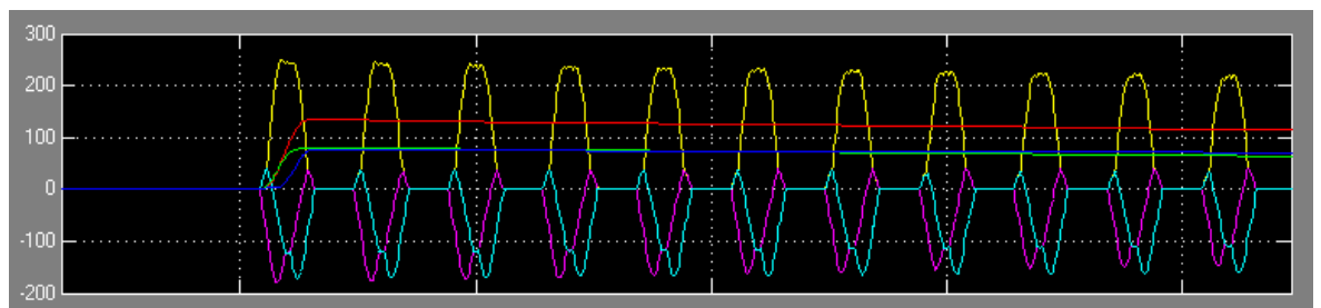
Figure. 5.4.10 - 119. Example of transformer magnetizing inrush currents.
