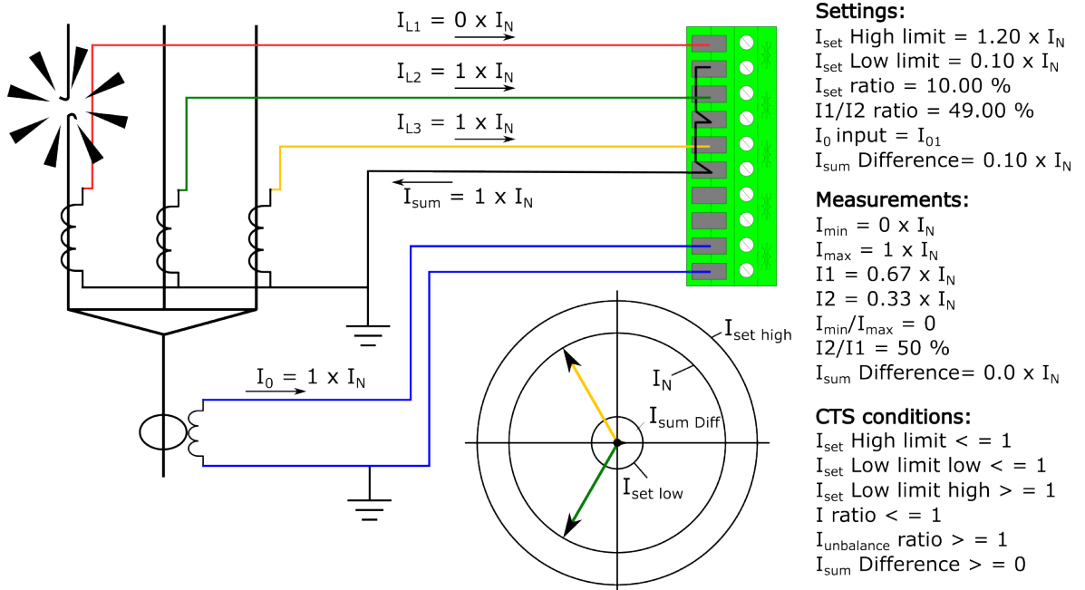
Figure. 5.6.1 - 149. Broken primary phase current wiring.
