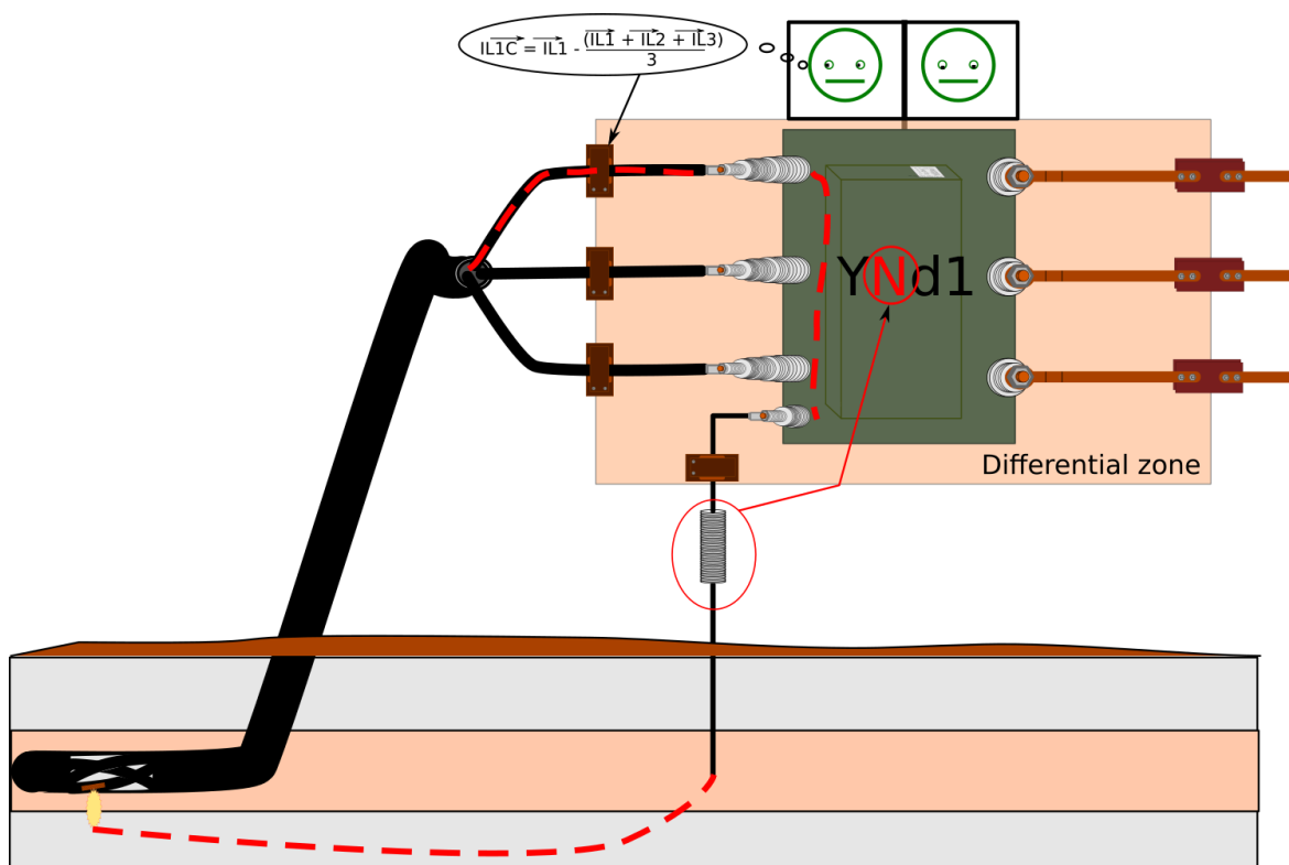
Figure. 5.4.10 - 115. Transformer earthing settings that compensates for external earth faults.
