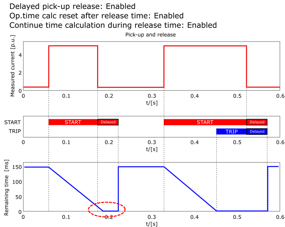
Figure. 5.4.1 - 66. Delayed pick-up release, delay counter value is decreasing during the release time.
