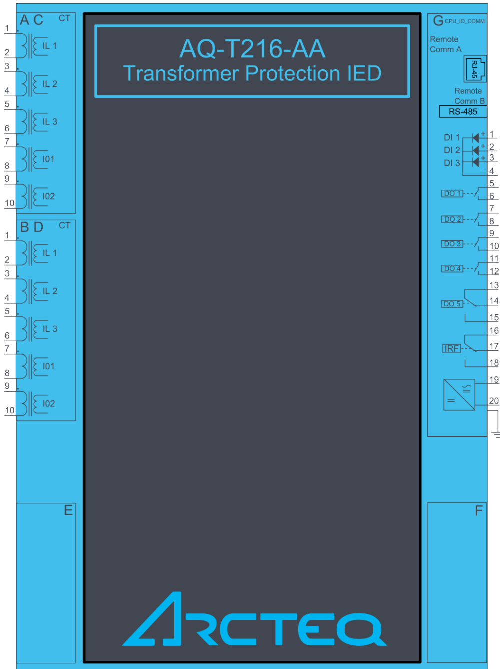
Figure. 7.1 - 159. AQ-T216 variant without add-on modules.
