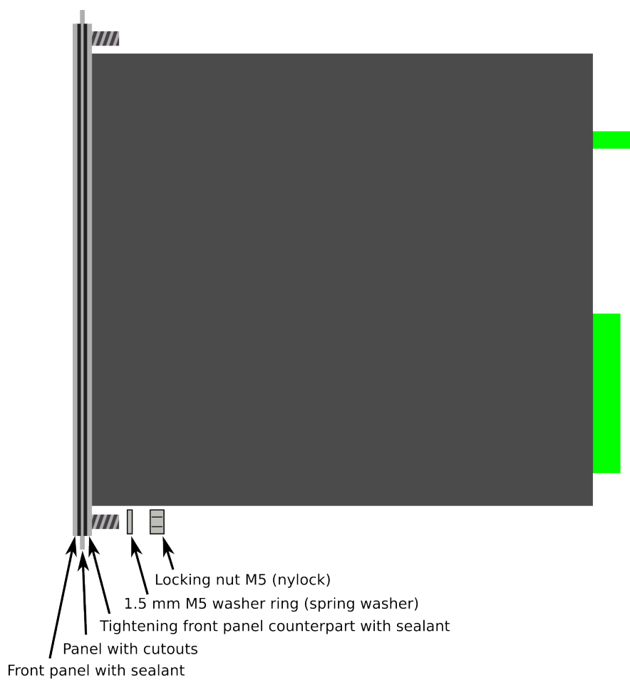
Figure. 8.13 - 187. Device installation.
