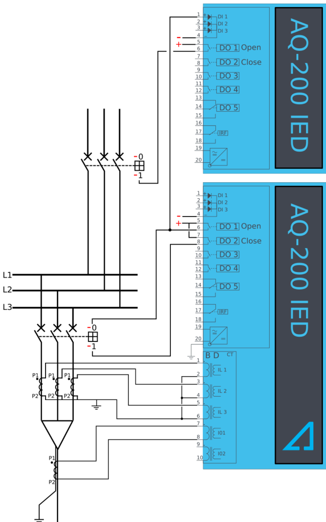
Figure. 5.4.6 - 81. Wiring diagram when the device is configured as a dedicated CBFP unit.
