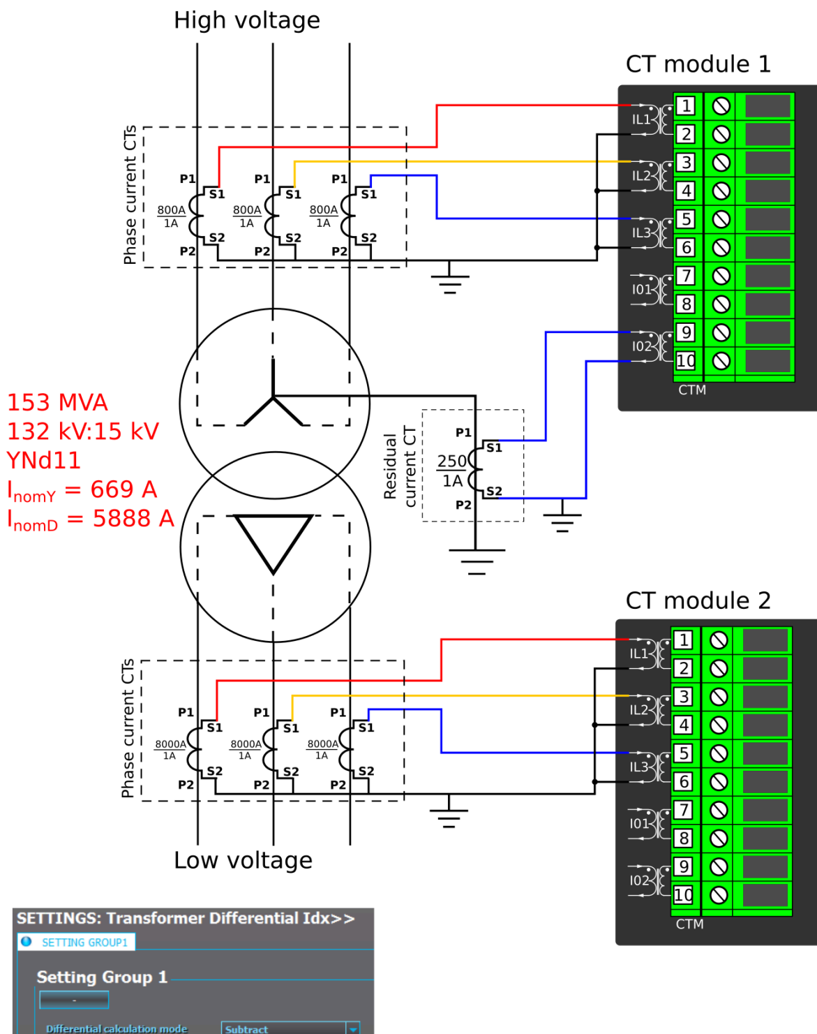
Figure. 5.2.1 - 53. Connections (application 1).
