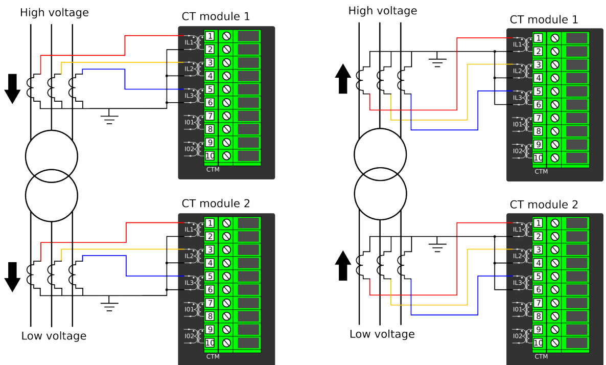
Figure. 5.4.10 - 106. CTs' starpoints requiring the "Subtract" mode.
