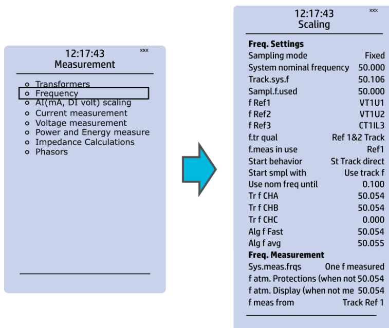
Figure. 4.7 - 43. Frequency submenu.
