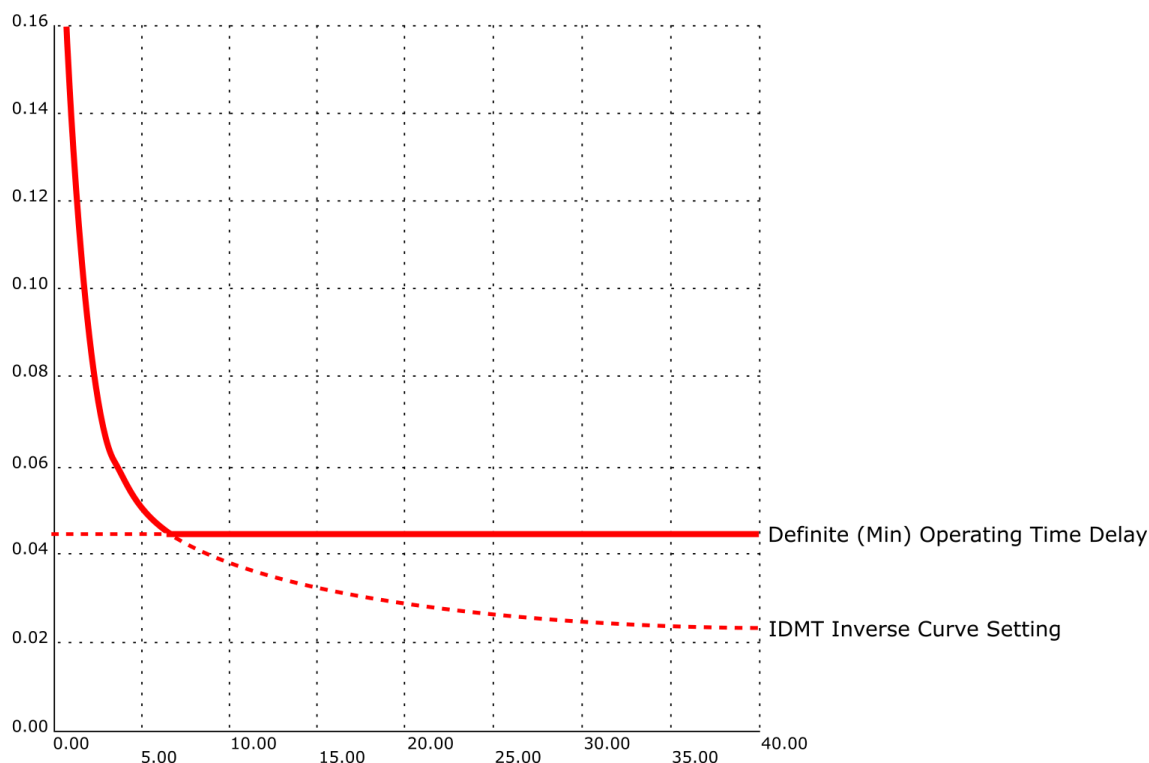
Figure. 5.4.1 - 61. Operating time delay: Definite (Min) and the minimum for tripping.
